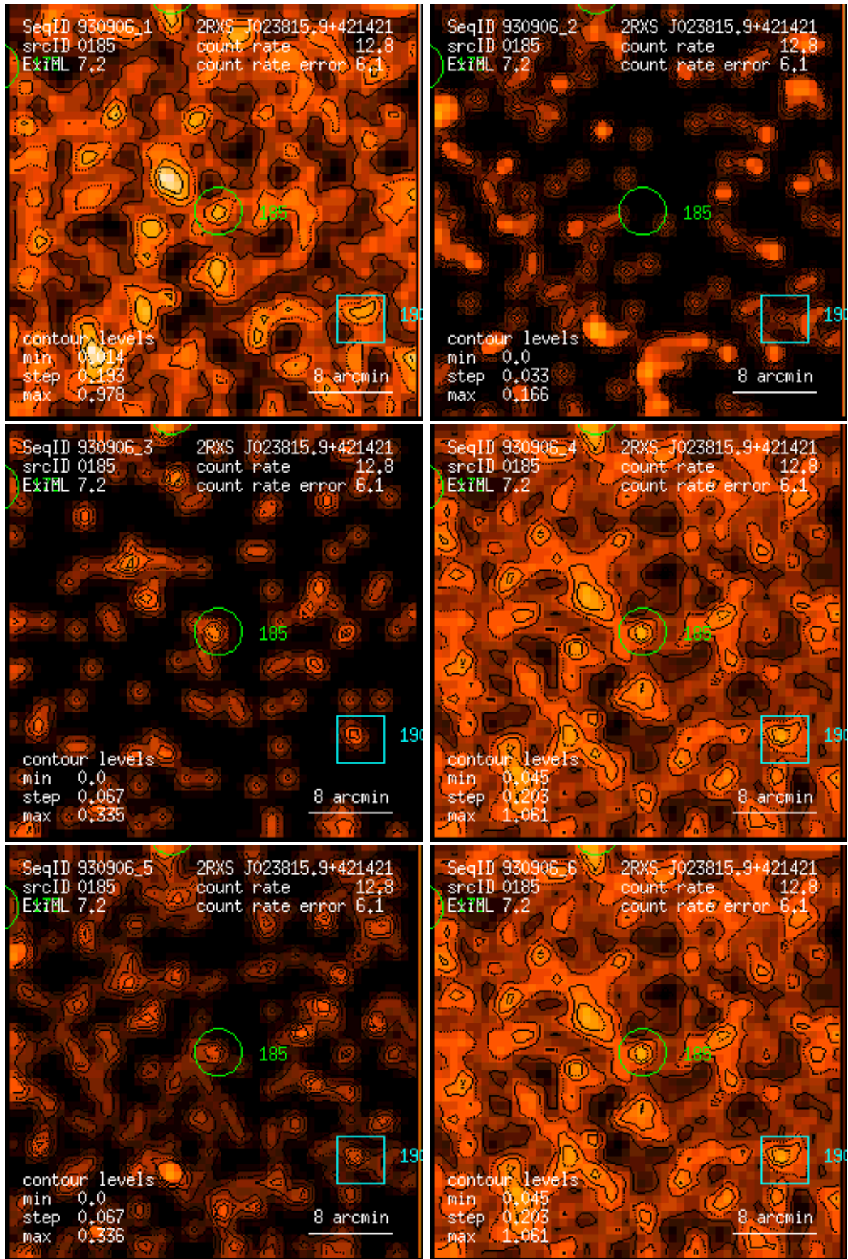
Figure 185: RASS 930906: detection 0185: band rate images, Gaussian filter: (1) PSPC channels 11 – 41, (2) 52 – 90, (3) 91 – 201, (4) 11 – 235, (5) 52 – 201, (6) 11 – 201. Broad band rates in counts/ks. Band rate contour levels in counts/ks/arcmin 2 .
