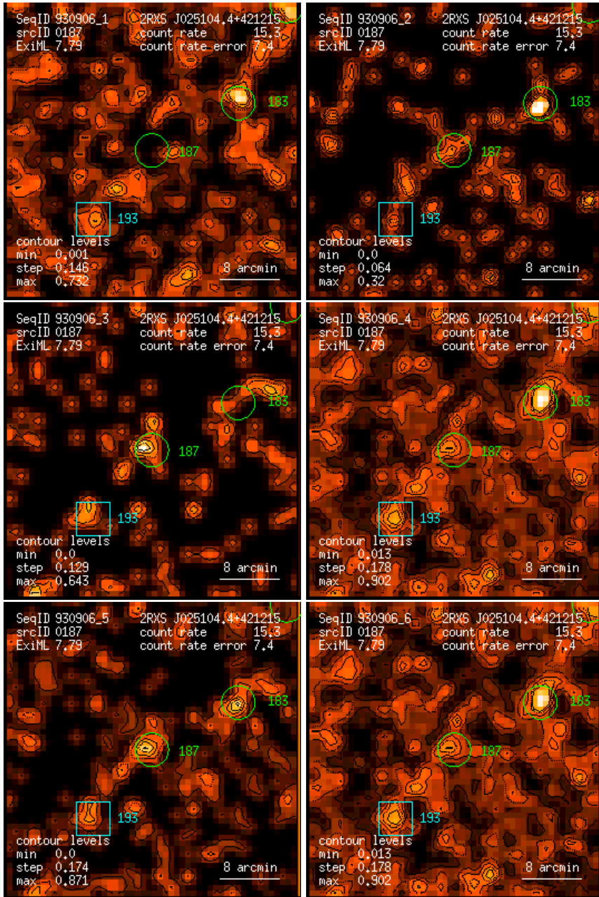
Figure 187: RASS 930906: detection 0187: band rate images, Gaussian filter: (1) PSPC channels 11 – 41, (2) 52 – 90, (3) 91 – 201, (4) 11 – 235, (5) 52 – 201, (6) 11 – 201. Broad band rates in counts/ks. Band rate contour levels in counts/ks/arcmin 2 .
