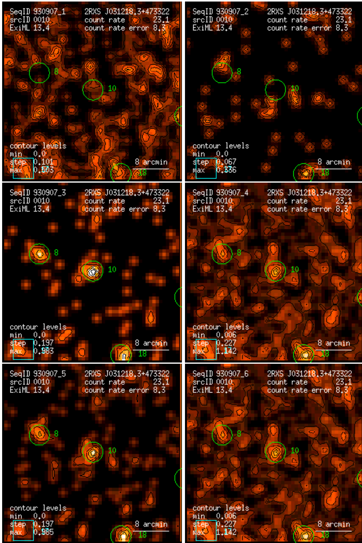
Figure 10: RASS 930907: detection 0010: band rate images, Gaussian filter: (1) PSPC channels 11 – 41, (2) 52 – 90, (3) 91 – 201, (4) 11 – 235, (5) 52 – 201, (6) 11 – 201. Broad band rates in counts/ks. Band rate contour levels in counts/ks/arcmin 2 .
