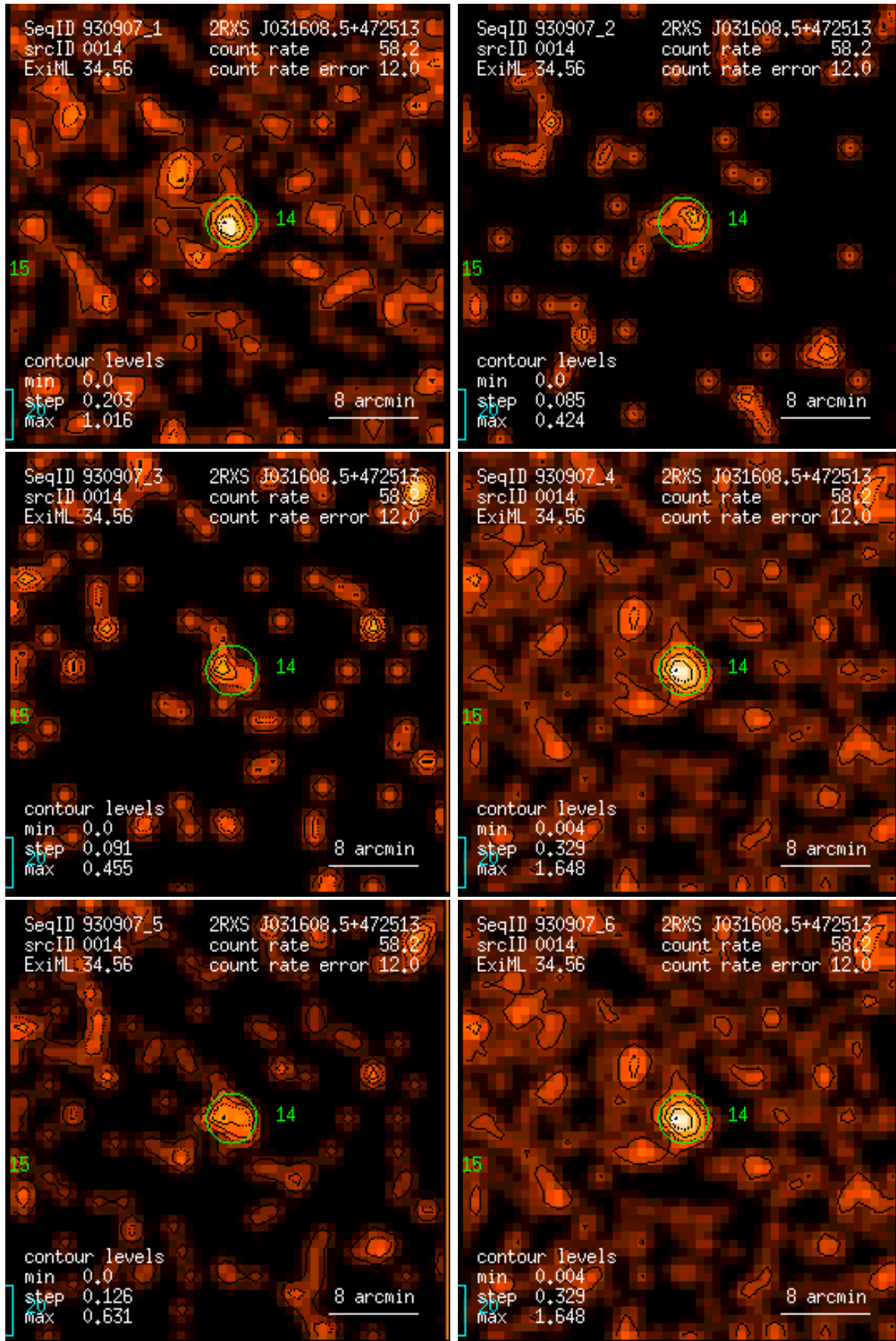
Figure 14: RASS 930907: detection 0014: band rate images, Gaussian filter: (1) PSPC channels 11 – 41, (2) 52 – 90, (3) 91 – 201, (4) 11 – 235, (5) 52 – 201, (6) 11 – 201. Broad band rates in counts/ks. Band rate contour levels in counts/ks/arcmin 2 .
