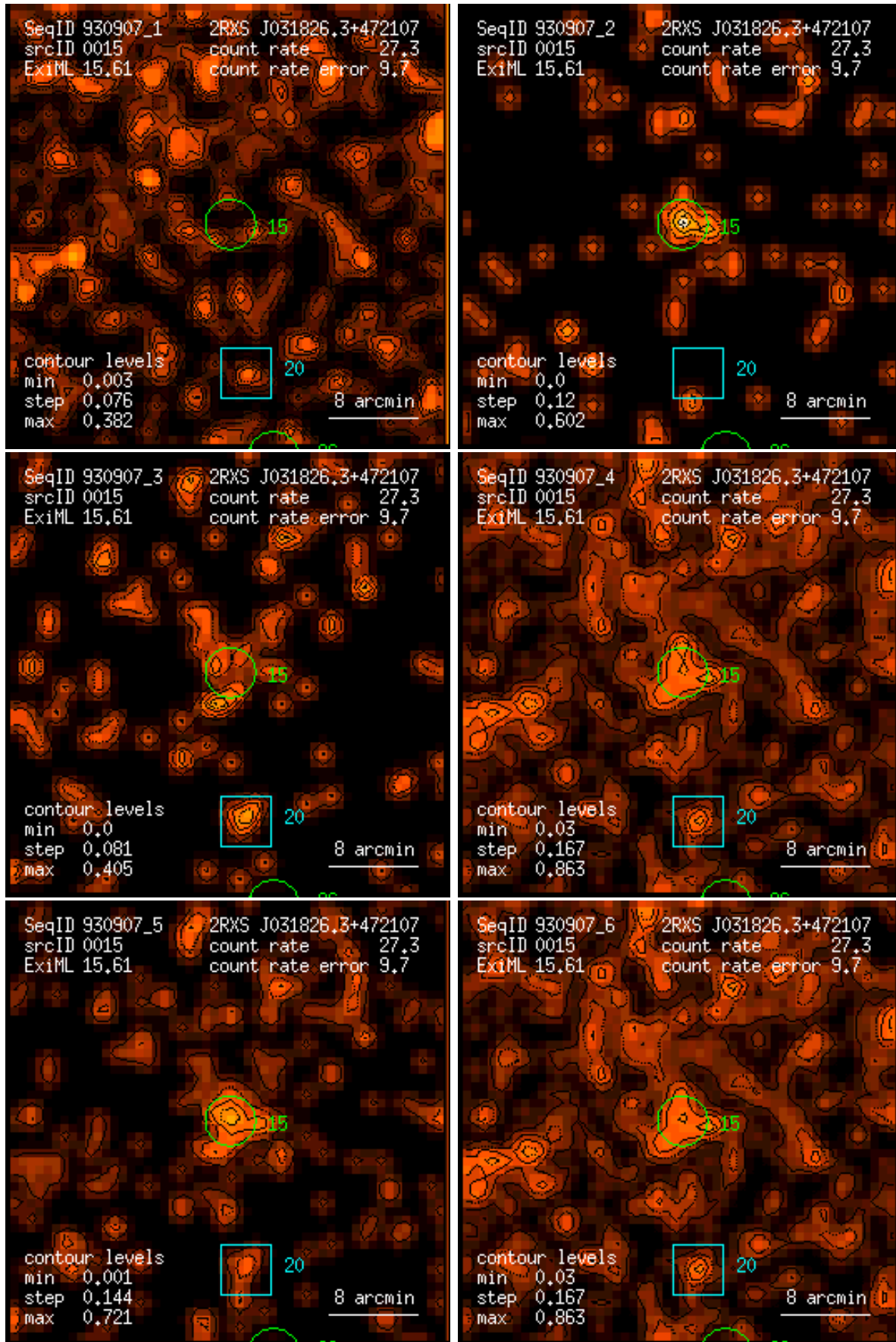
Figure 15: RASS 930907: detection 0015: band rate images, Gaussian filter: (1) PSPC channels 11 – 41, (2) 52 – 90, (3) 91 – 201, (4) 11 – 235, (5) 52 – 201, (6) 11 – 201. Broad band rates in counts/ks. Band rate contour levels in counts/ks/arcmin 2 .
