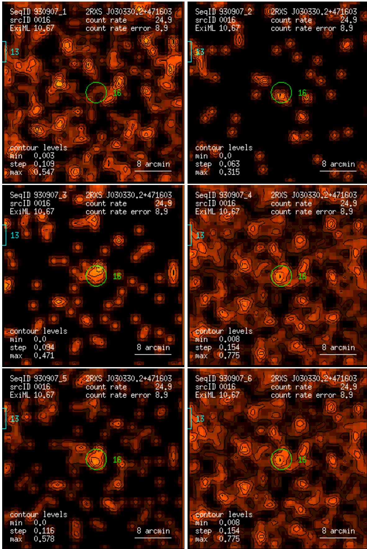
Figure 16: RASS 930907: detection 0016: band rate images, Gaussian filter: (1) PSPC channels 11 – 41, (2) 52 – 90, (3) 91 – 201, (4) 11 – 235, (5) 52 – 201, (6) 11 – 201. Broad band rates in counts/ks. Band rate contour levels in counts/ks/arcmin 2 .
