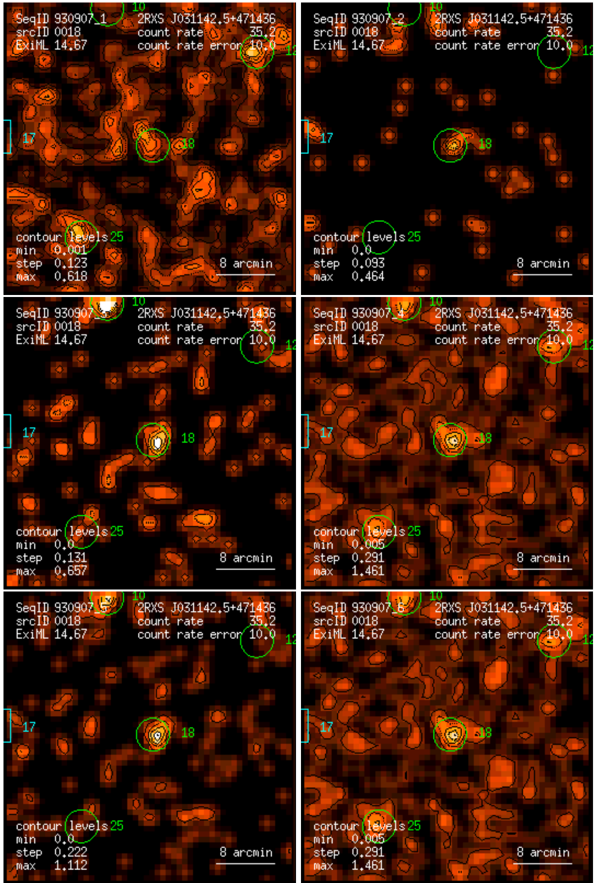
Figure 18: RASS 930907: detection 0018: band rate images, Gaussian filter: (1) PSPC channels 11 – 41, (2) 52 – 90, (3) 91 – 201, (4) 11 – 235, (5) 52 – 201, (6) 11 – 201. Broad band rates in counts/ks. Band rate contour levels in counts/ks/arcmin 2 .
