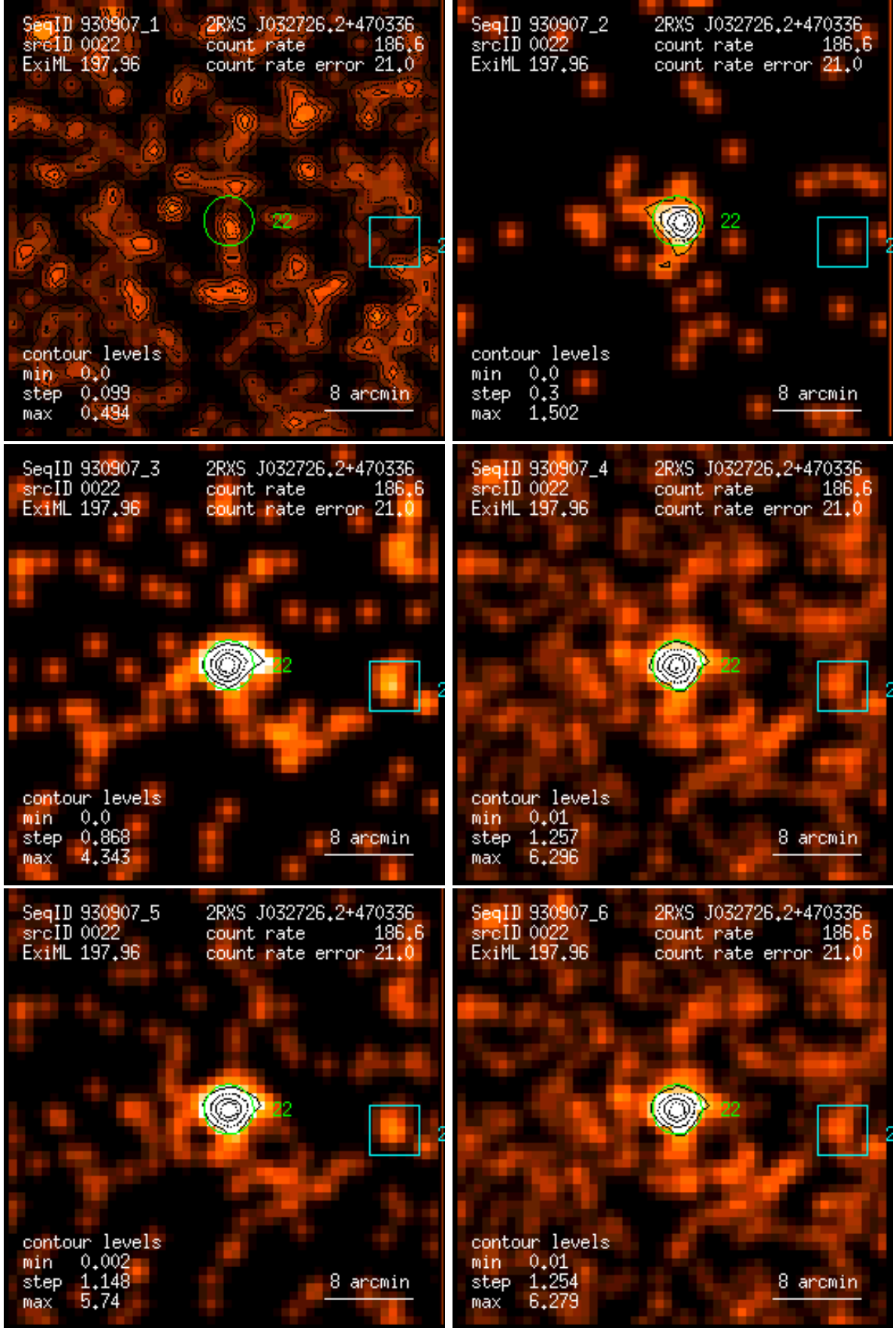
Figure 22: RASS 930907: detection 0022: band rate images, Gaussian filter: (1) PSPC channels 11 – 41, (2) 52 – 90, (3) 91 – 201, (4) 11 – 235, (5) 52 – 201, (6) 11 – 201. Broad band rates in counts/ks. Band rate contour levels in counts/ks/arcmin 2 .
