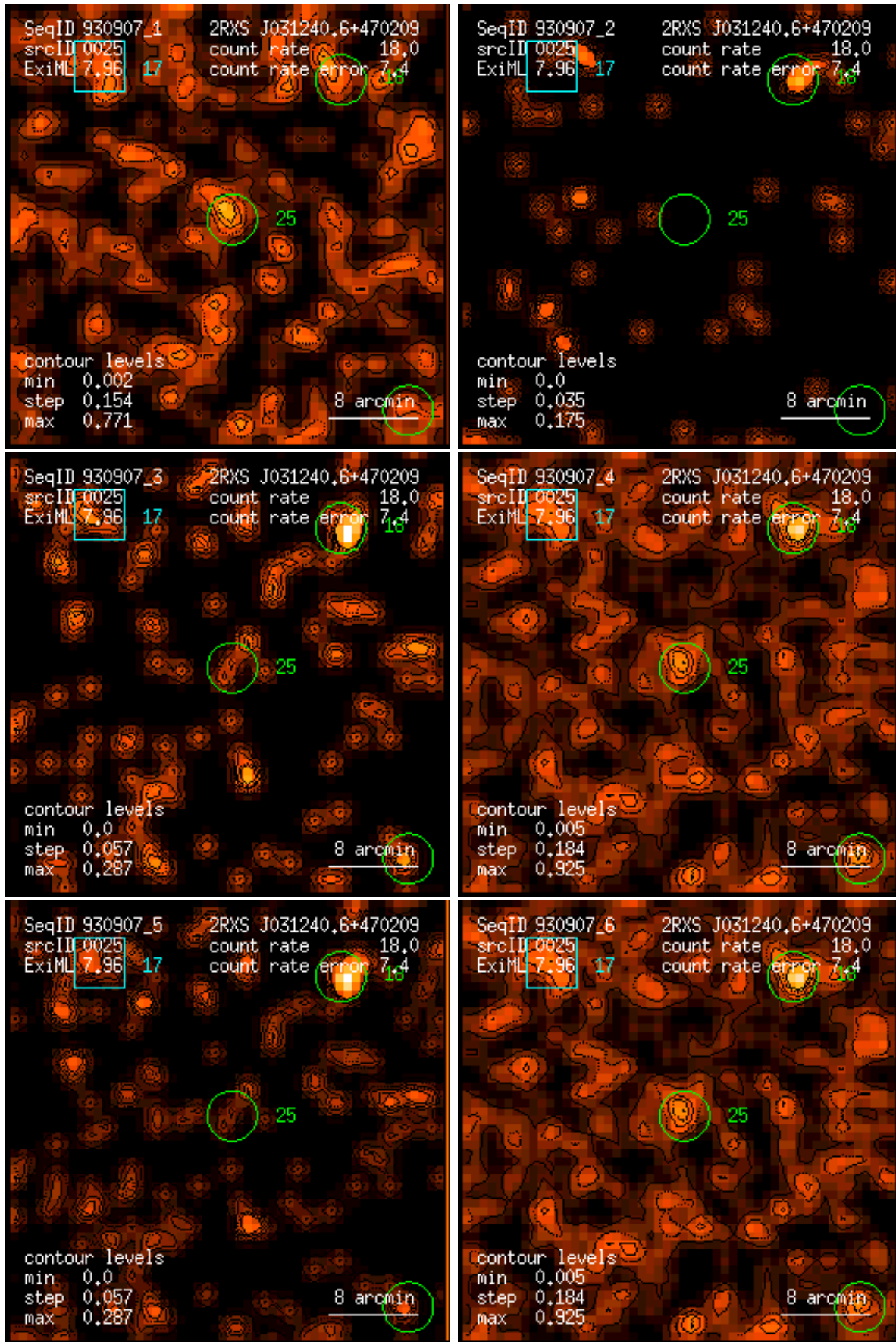
Figure 25: RASS 930907: detection 0025: band rate images, Gaussian filter: (1) PSPC channels 11 – 41, (2) 52 – 90, (3) 91 – 201, (4) 11 – 235, (5) 52 – 201, (6) 11 – 201. Broad band rates in counts/ks. Band rate contour levels in counts/ks/arcmin 2 .
