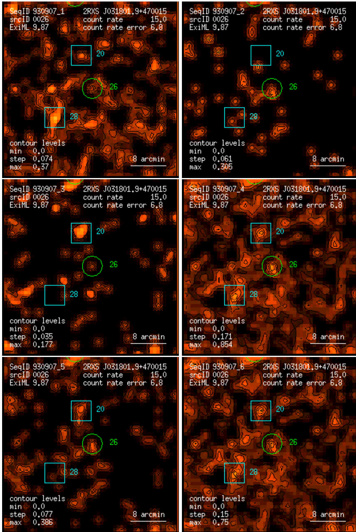
Figure 26: RASS 930907: detection 0026: band rate images, Gaussian filter: (1) PSPC channels 11 – 41, (2) 52 – 90, (3) 91 – 201, (4) 11 – 235, (5) 52 – 201, (6) 11 – 201. Broad band rates in counts/ks. Band rate contour levels in counts/ks/arcmin 2 .
