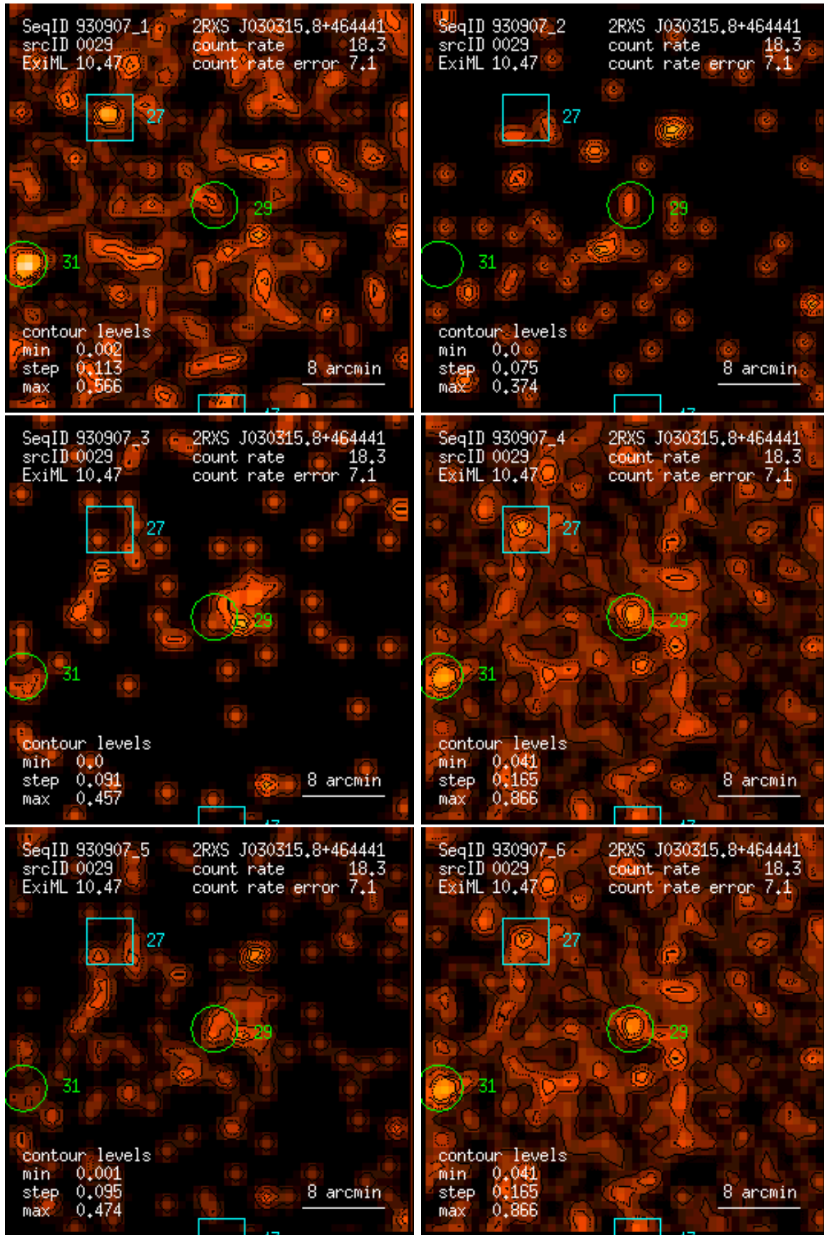
Figure 29: RASS 930907: detection 0029: band rate images, Gaussian filter: (1) PSPC channels 11 – 41, (2) 52 – 90, (3) 91 – 201, (4) 11 – 235, (5) 52 – 201, (6) 11 – 201. Broad band rates in counts/ks. Band rate contour levels in counts/ks/arcmin 2 .
