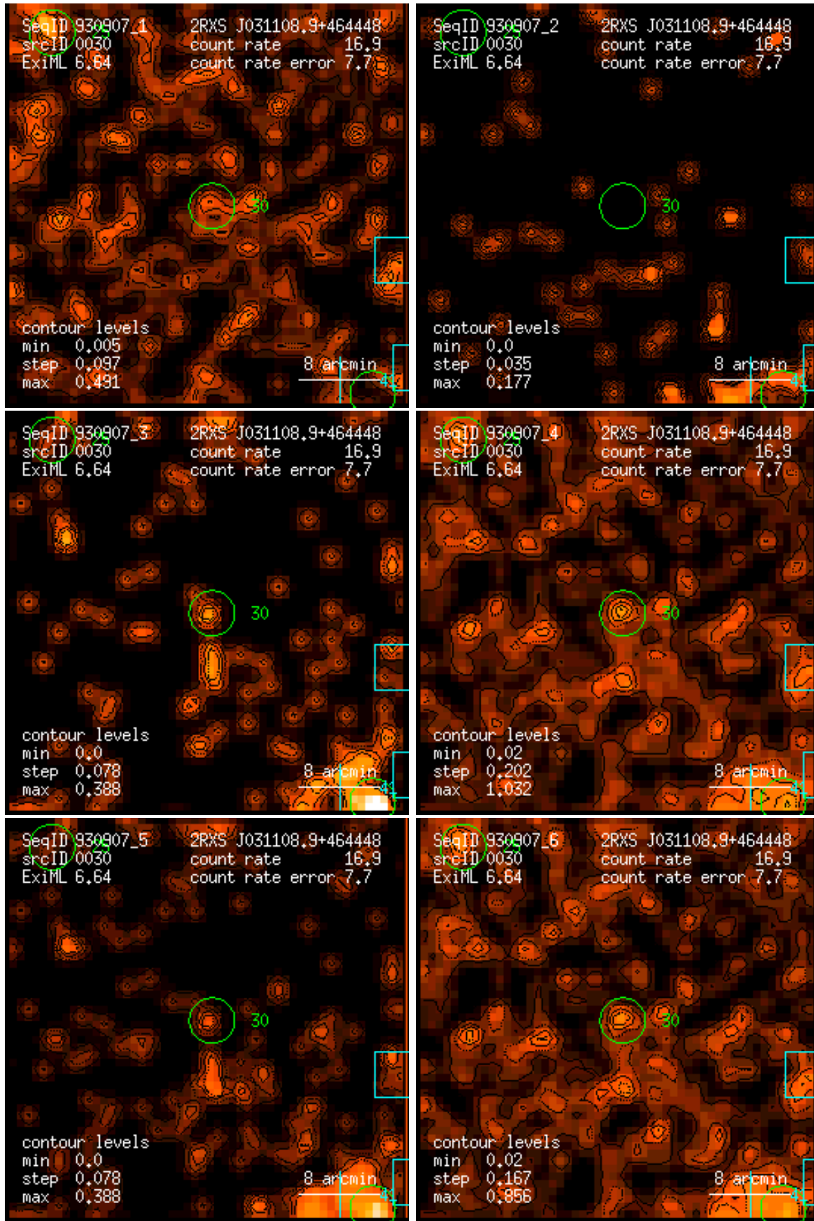
Figure 30: RASS 930907: detection 0030: band rate images, Gaussian filter: (1) PSPC channels 11 – 41, (2) 52 – 90, (3) 91 – 201, (4) 11 – 235, (5) 52 – 201, (6) 11 – 201. Broad band rates in counts/ks. Band rate contour levels in counts/ks/arcmin 2 .
