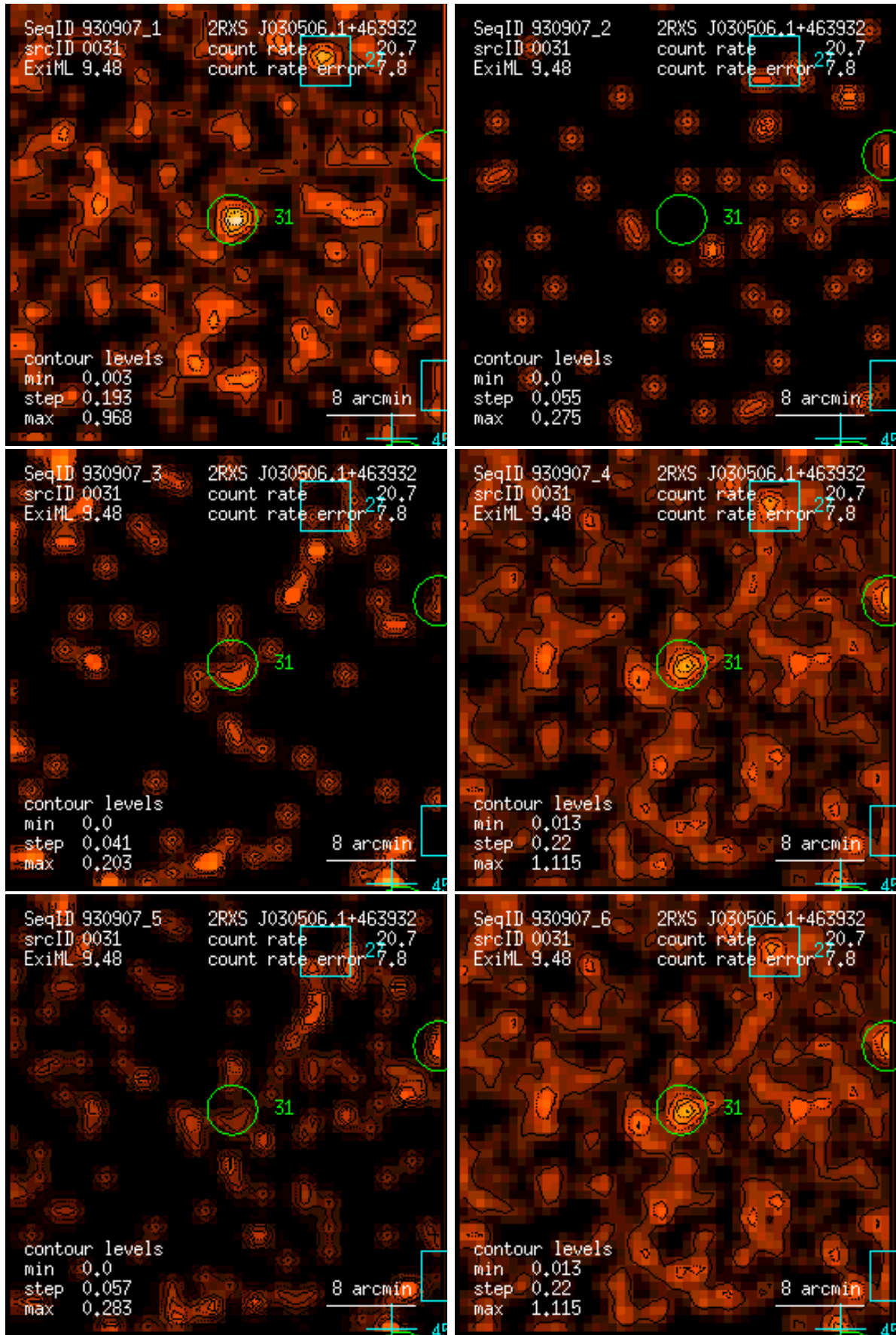
Figure 31: RASS 930907: detection 0031: band rate images, Gaussian filter: (1) PSPC channels 11 – 41, (2) 52 – 90, (3) 91 – 201, (4) 11 – 235, (5) 52 – 201, (6) 11 – 201. Broad band rates in counts/ks. Band rate contour levels in counts/ks/arcmin 2 .
