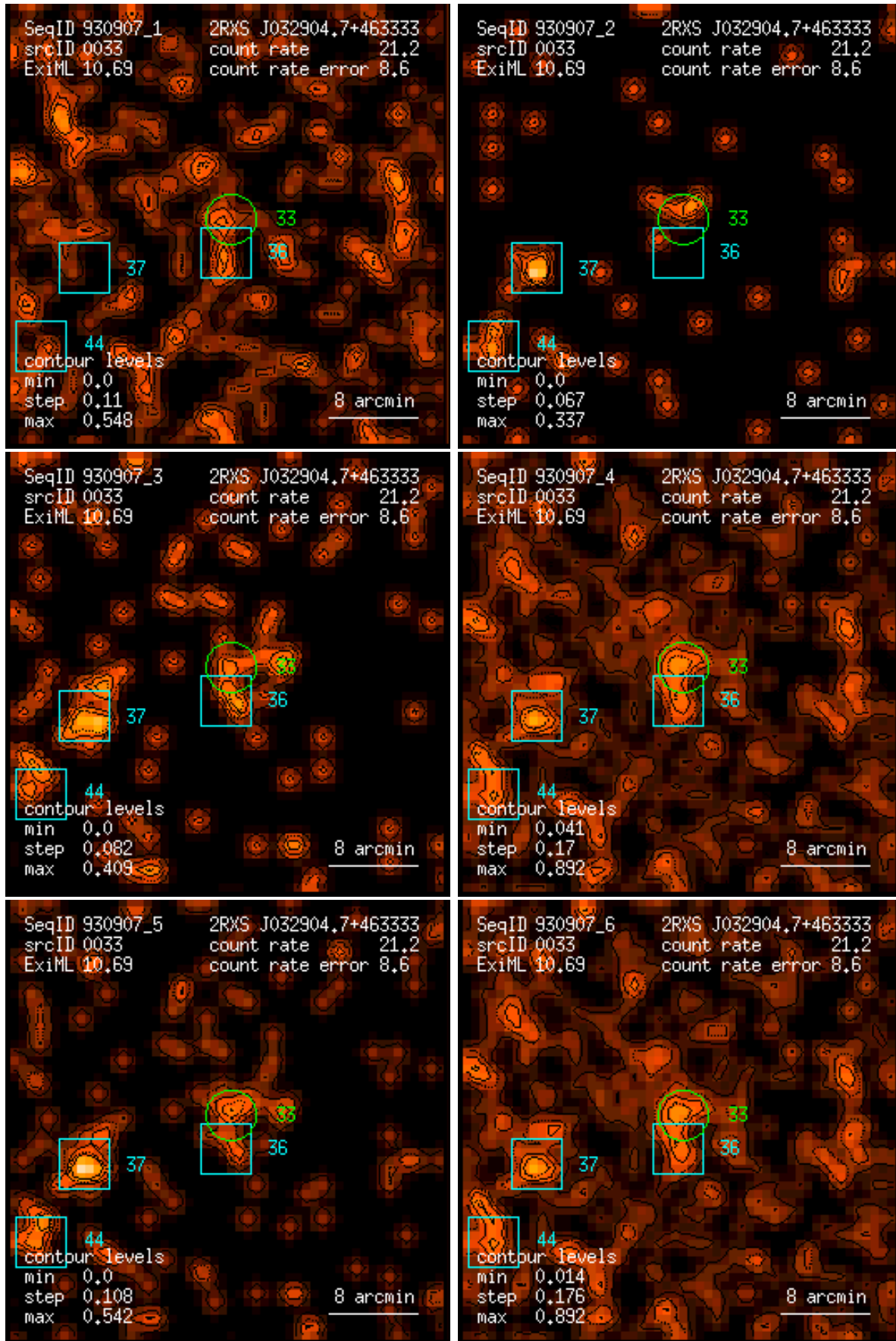
Figure 33: RASS 930907: detection 0033: band rate images, Gaussian filter: (1) PSPC channels 11 – 41, (2) 52 – 90, (3) 91 – 201, (4) 11 – 235, (5) 52 – 201, (6) 11 – 201. Broad band rates in counts/ks. Band rate contour levels in counts/ks/arcmin 2 .
