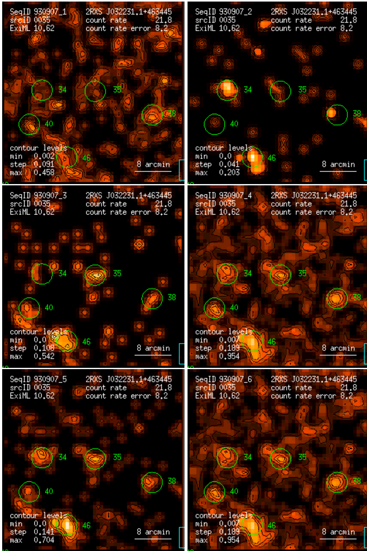
Figure 35: RASS 930907: detection 0035: band rate images, Gaussian filter: (1) PSPC channels 11 – 41, (2) 52 – 90, (3) 91 – 201, (4) 11 – 235, (5) 52 – 201, (6) 11 – 201. Broad band rates in counts/ks. Band rate contour levels in counts/ks/arcmin 2 .
