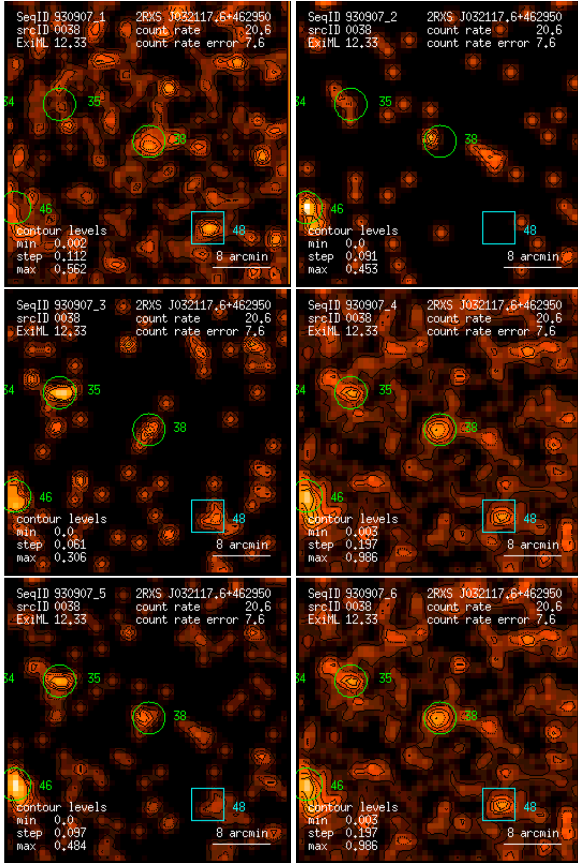
Figure 38: RASS 930907: detection 0038: band rate images, Gaussian filter: (1) PSPC channels 11 – 41, (2) 52 – 90, (3) 91 – 201, (4) 11 – 235, (5) 52 – 201, (6) 11 – 201. Broad band rates in counts/ks. Band rate contour levels in counts/ks/arcmin 2 .
