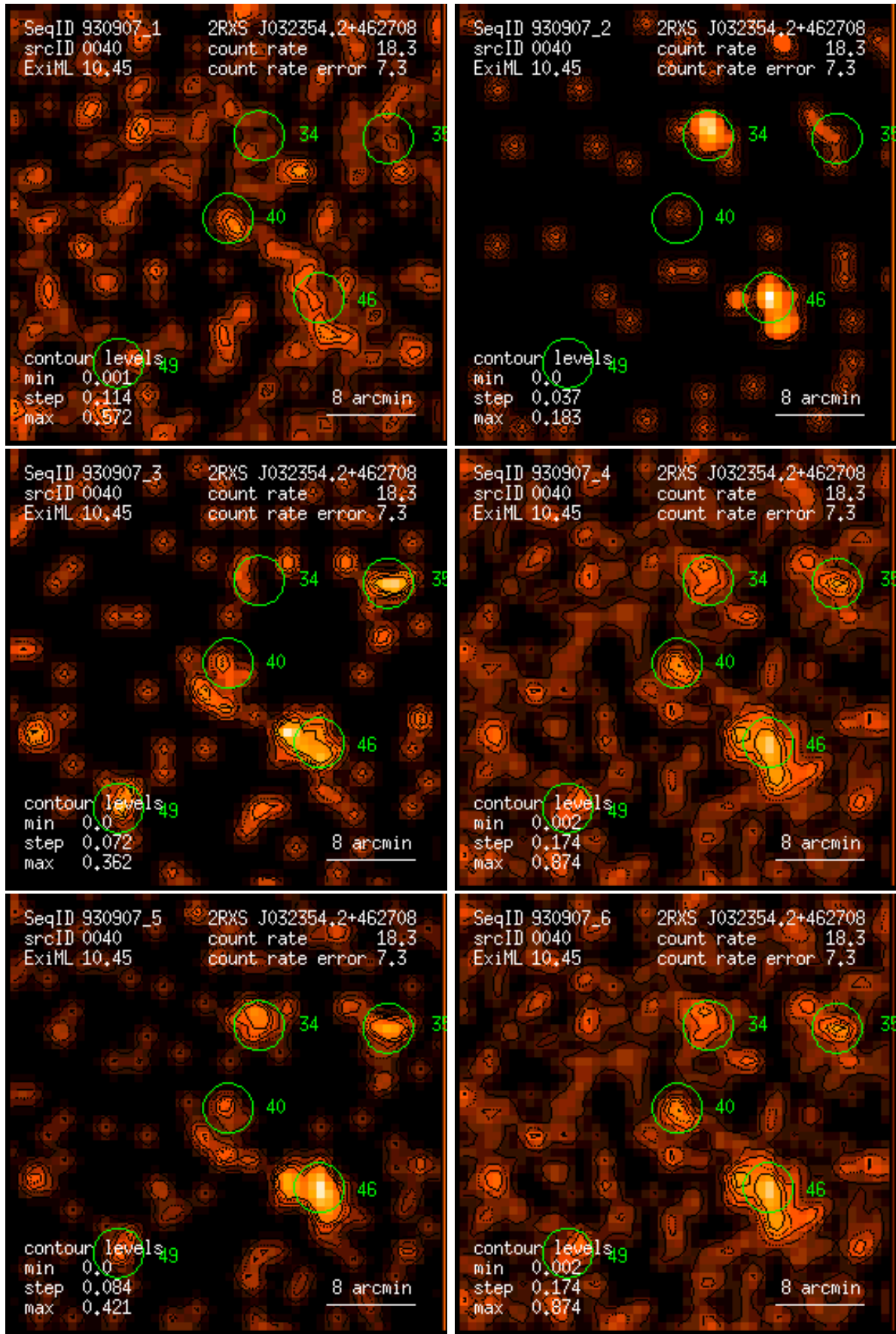
Figure 40: RASS 930907: detection 0040: band rate images, Gaussian filter: (1) PSPC channels 11 – 41, (2) 52 – 90, (3) 91 – 201, (4) 11 – 235, (5) 52 – 201, (6) 11 – 201. Broad band rates in counts/ks. Band rate contour levels in counts/ks/arcmin 2 .
