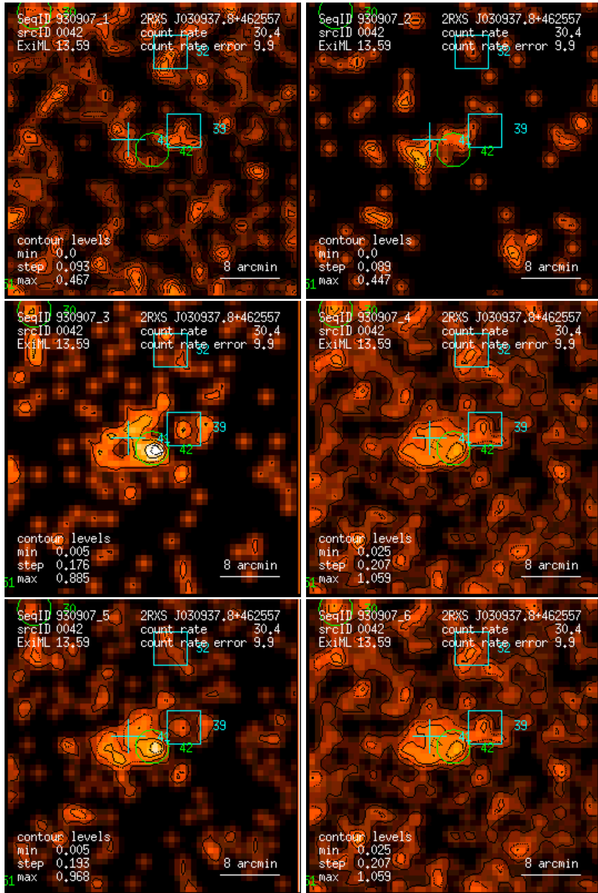
Figure 42: RASS 930907: detection 0042: band rate images, Gaussian filter: (1) PSPC channels 11 – 41, (2) 52 – 90, (3) 91 – 201, (4) 11 – 235, (5) 52 – 201, (6) 11 – 201. Broad band rates in counts/ks. Band rate contour levels in counts/ks/arcmin 2 .
