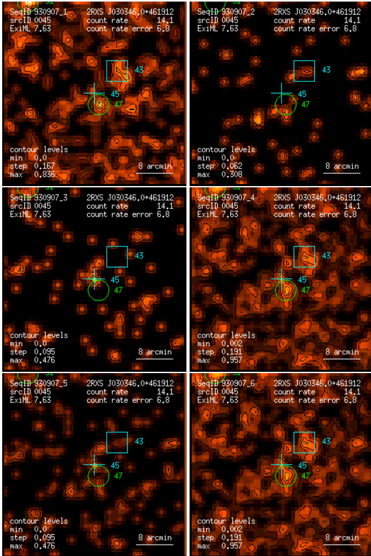
Figure 45: RASS 930907: detection 0045: band rate images, Gaussian filter: (1) PSPC channels 11 – 41, (2) 52 – 90, (3) 91 – 201, (4) 11 – 235, (5) 52 – 201, (6) 11 – 201. Broad band rates in counts/ks. Band rate contour levels in counts/ks/arcmin 2 .
