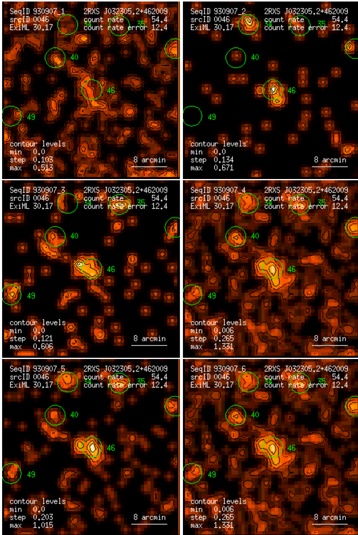
Figure 46: RASS 930907: detection 0046: band rate images, Gaussian filter: (1) PSPC channels 11 – 41, (2) 52 – 90, (3) 91 – 201, (4) 11 – 235, (5) 52 – 201, (6) 11 – 201. Broad band rates in counts/ks. Band rate contour levels in counts/ks/arcmin 2 .
