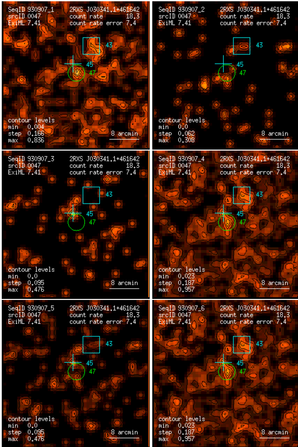
Figure 47: RASS 930907: detection 0047: band rate images, Gaussian filter: (1) PSPC channels 11 – 41, (2) 52 – 90, (3) 91 – 201, (4) 11 – 235, (5) 52 – 201, (6) 11 – 201. Broad band rates in counts/ks. Band rate contour levels in counts/ks/arcmin 2 .
