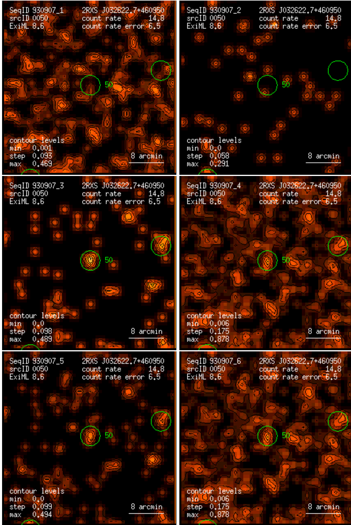
Figure 50: RASS 930907: detection 0050: band rate images, Gaussian filter: (1) PSPC channels 11 – 41, (2) 52 – 90, (3) 91 – 201, (4) 11 – 235, (5) 52 – 201, (6) 11 – 201. Broad band rates in counts/ks. Band rate contour levels in counts/ks/arcmin 2 .
