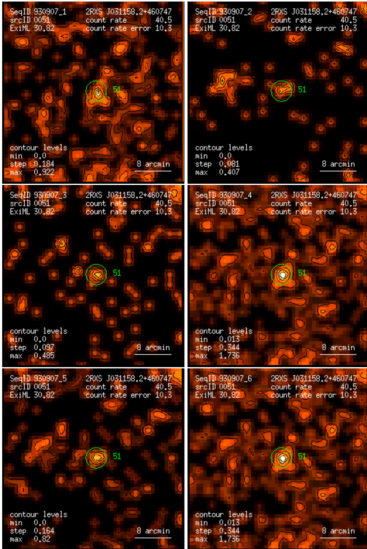
Figure 51: RASS 930907: detection 0051: band rate images, Gaussian filter: (1) PSPC channels 11 – 41, (2) 52 – 90, (3) 91 – 201, (4) 11 – 235, (5) 52 – 201, (6) 11 – 201. Broad band rates in counts/ks. Band rate contour levels in counts/ks/arcmin 2 .
