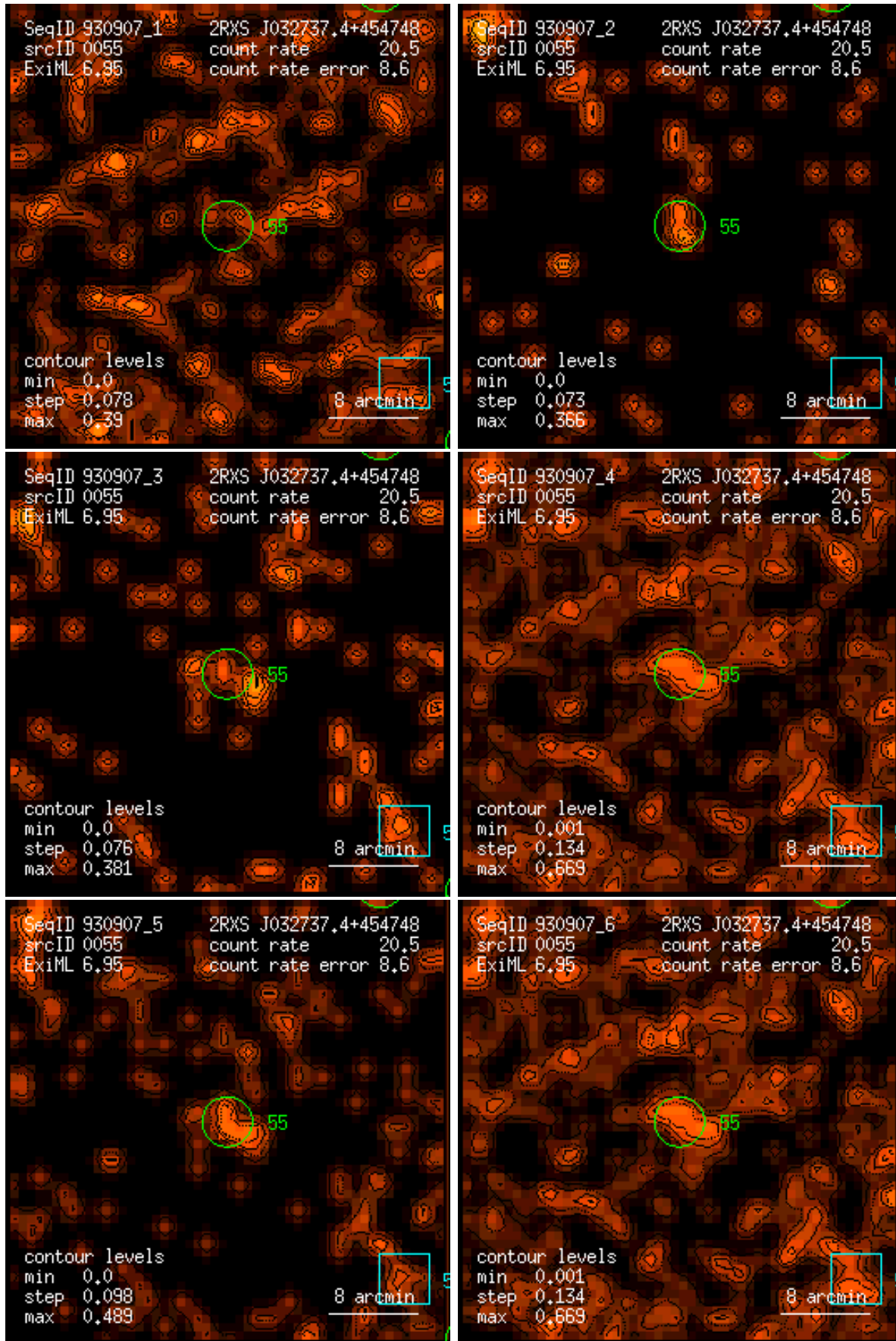
Figure 55: RASS 930907: detection 0055: band rate images, Gaussian filter: (1) PSPC channels 11 – 41, (2) 52 – 90, (3) 91 – 201, (4) 11 – 235, (5) 52 – 201, (6) 11 – 201. Broad band rates in counts/ks. Band rate contour levels in counts/ks/arcmin 2 .
