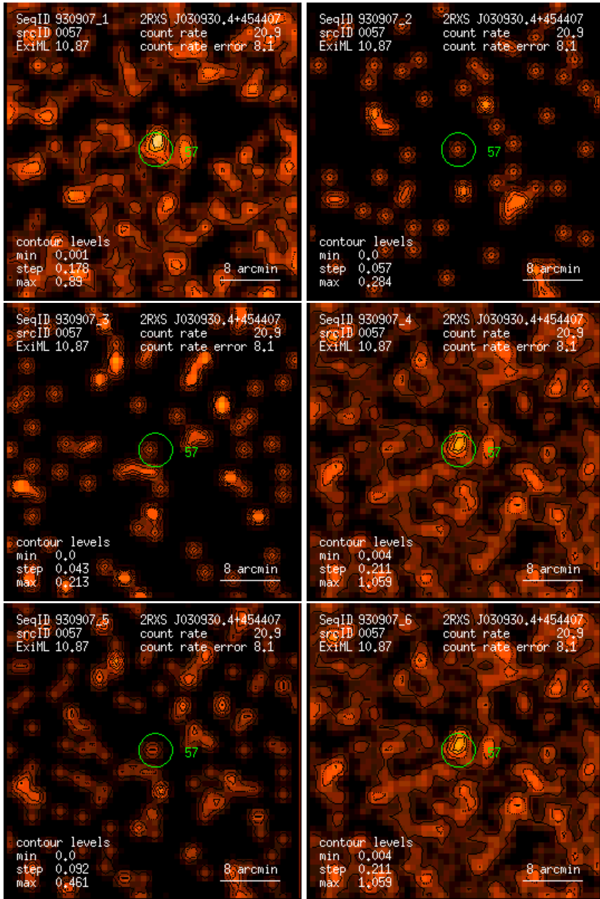
Figure 57: RASS 930907: detection 0057: band rate images, Gaussian filter: (1) PSPC channels 11 – 41, (2) 52 – 90, (3) 91 – 201, (4) 11 – 235, (5) 52 – 201, (6) 11 – 201. Broad band rates in counts/ks. Band rate contour levels in counts/ks/arcmin 2 .
