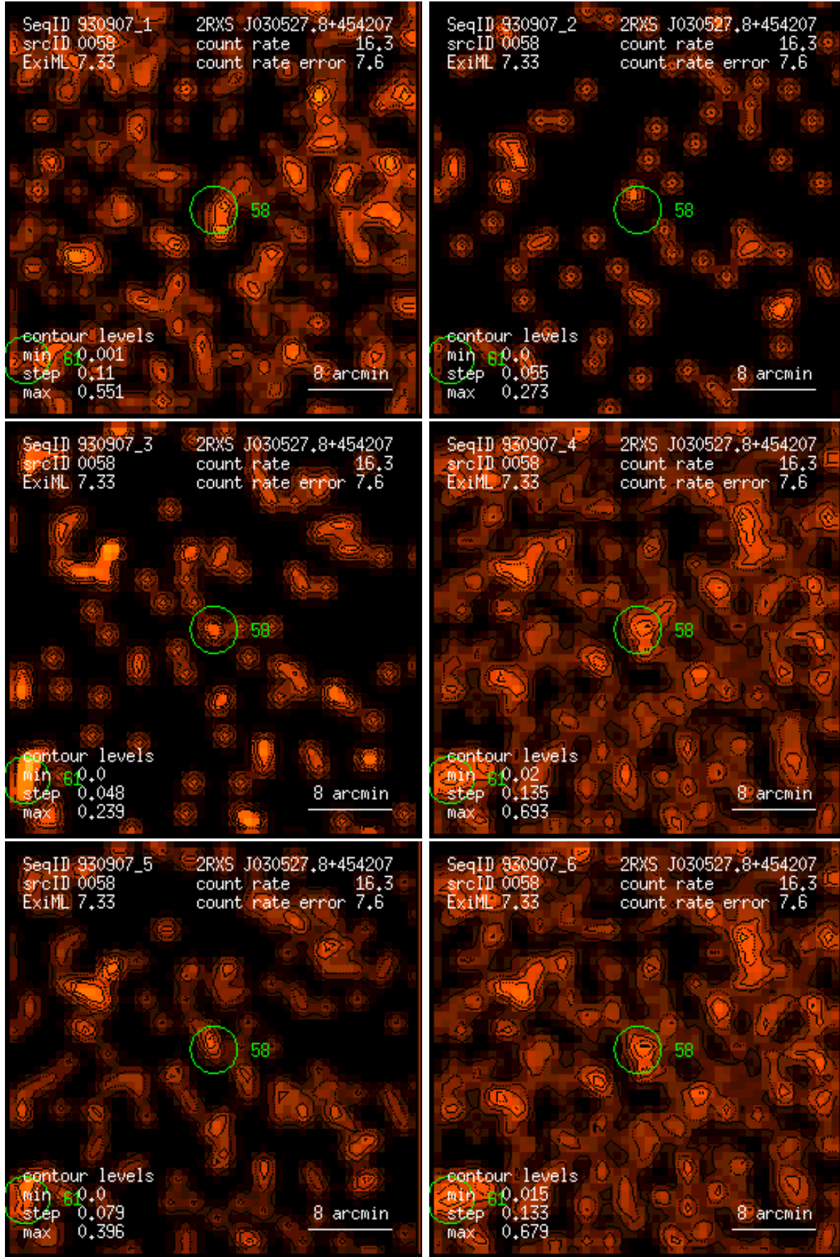
Figure 58: RASS 930907: detection 0058: band rate images, Gaussian filter: (1) PSPC channels 11 – 41, (2) 52 – 90, (3) 91 – 201, (4) 11 – 235, (5) 52 – 201, (6) 11 – 201. Broad band rates in counts/ks. Band rate contour levels in counts/ks/arcmin 2 .
