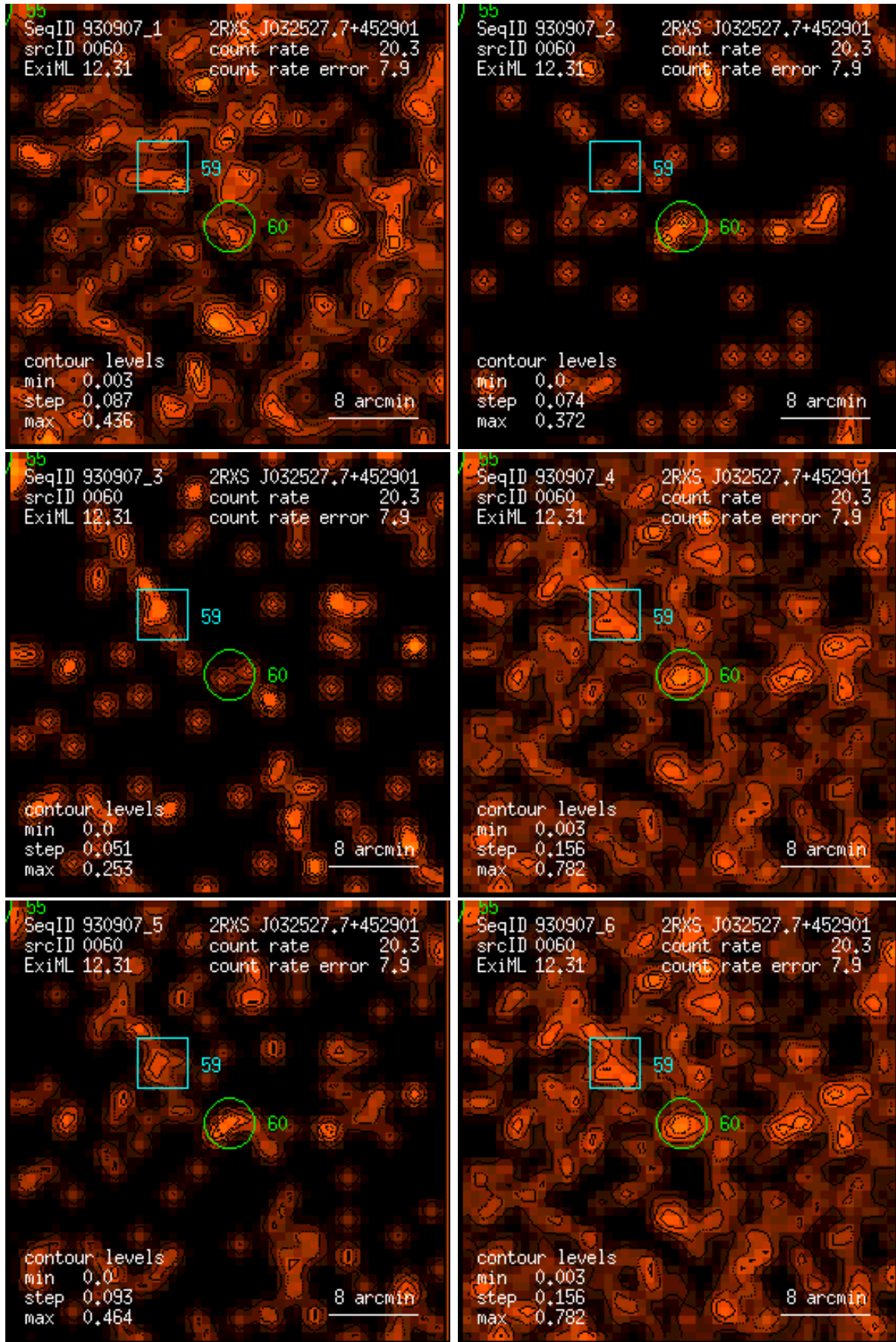
Figure 60: RASS 930907: detection 0060: band rate images, Gaussian filter: (1) PSPC channels 11 – 41, (2) 52 – 90, (3) 91 – 201, (4) 11 – 235, (5) 52 – 201, (6) 11 – 201. Broad band rates in counts/ks. Band rate contour levels in counts/ks/arcmin 2 .
