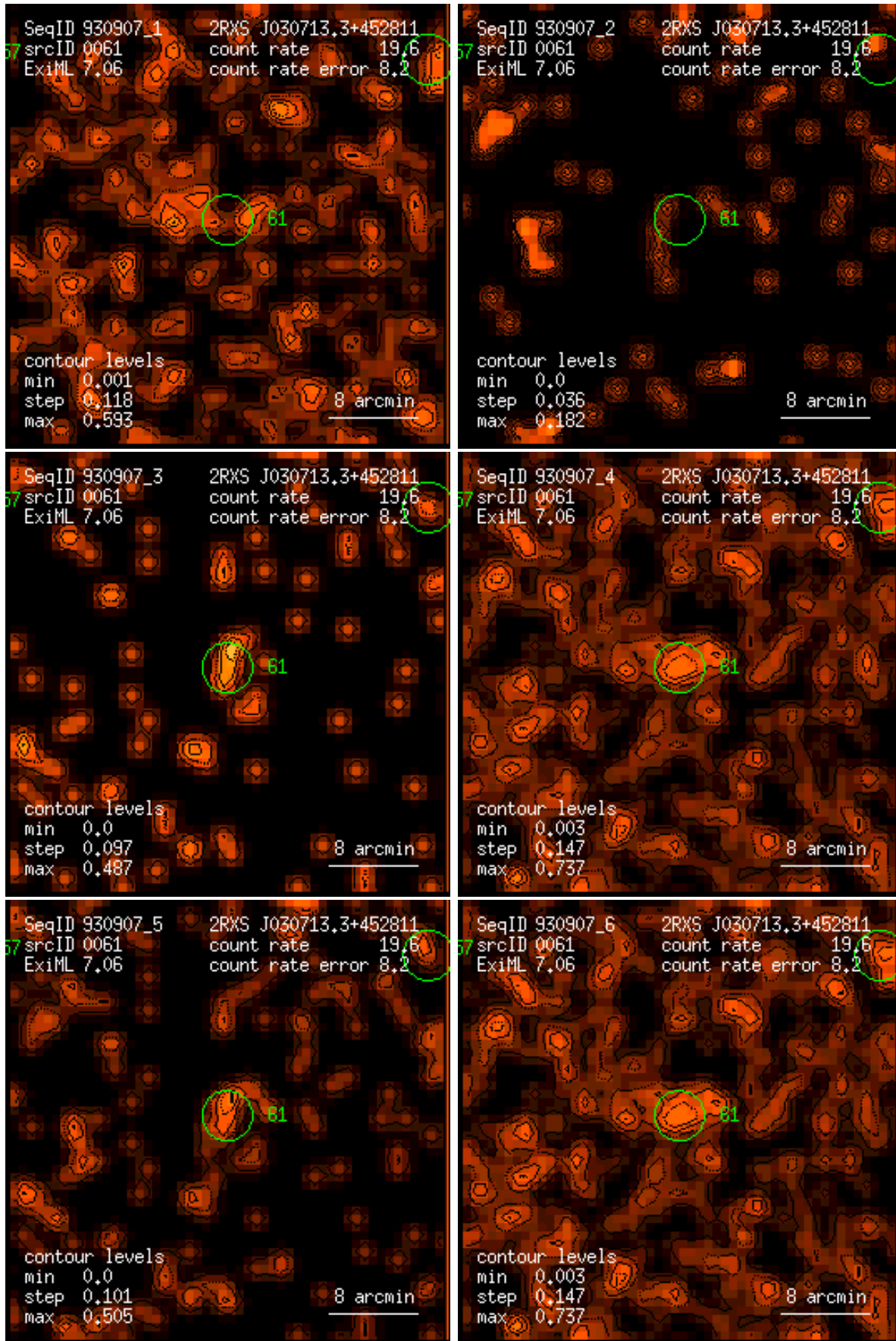
Figure 61: RASS 930907: detection 0061: band rate images, Gaussian filter: (1) PSPC channels 11 – 41, (2) 52 – 90, (3) 91 – 201, (4) 11 – 235, (5) 52 – 201, (6) 11 – 201. Broad band rates in counts/ks. Band rate contour levels in counts/ks/arcmin 2 .
