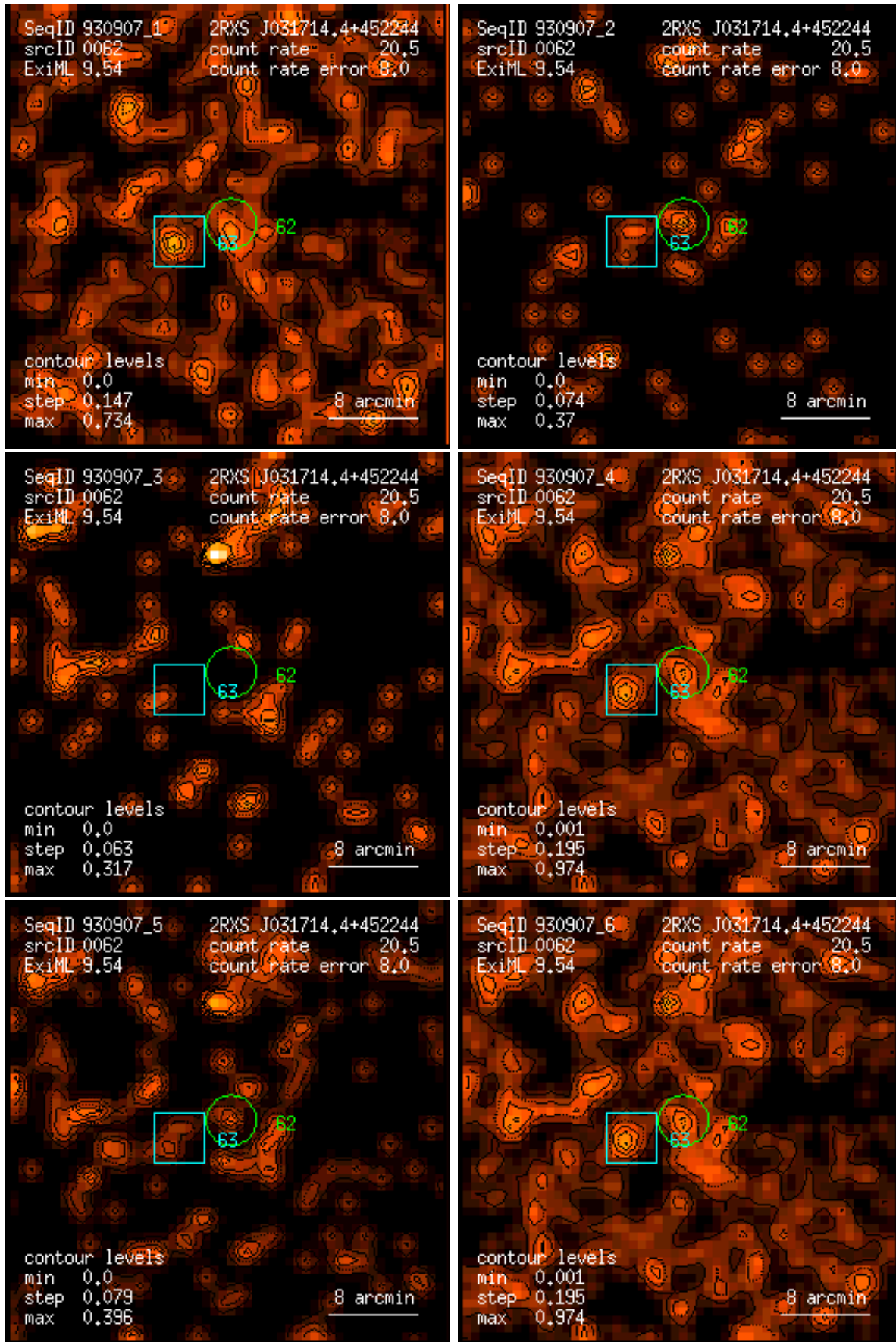
Figure 62: RASS 930907: detection 0062: band rate images, Gaussian filter: (1) PSPC channels 11 – 41, (2) 52 – 90, (3) 91 – 201, (4) 11 – 235, (5) 52 – 201, (6) 11 – 201. Broad band rates in counts/ks. Band rate contour levels in counts/ks/arcmin 2 .
