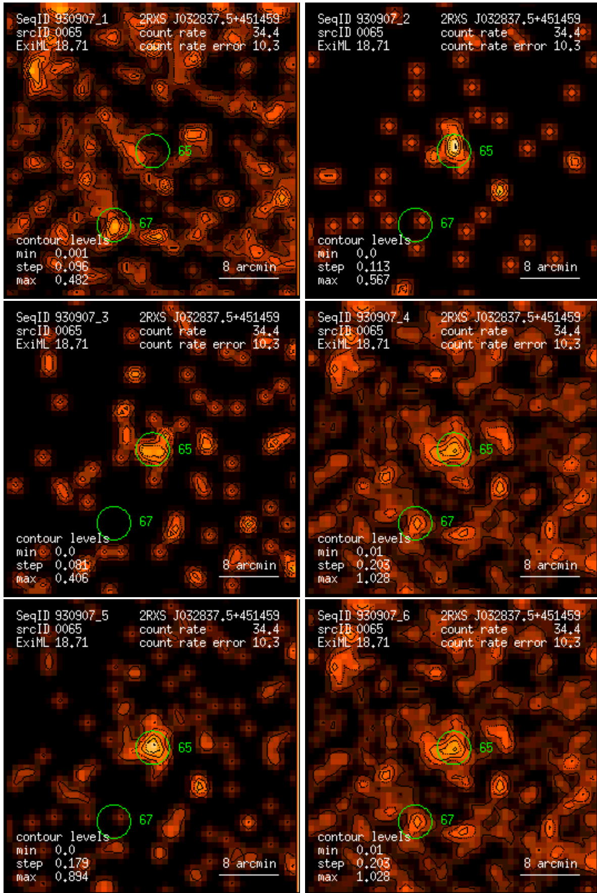
Figure 65: RASS 930907: detection 0065: band rate images, Gaussian filter: (1) PSPC channels 11 – 41, (2) 52 – 90, (3) 91 – 201, (4) 11 – 235, (5) 52 – 201, (6) 11 – 201. Broad band rates in counts/ks. Band rate contour levels in counts/ks/arcmin 2 .
