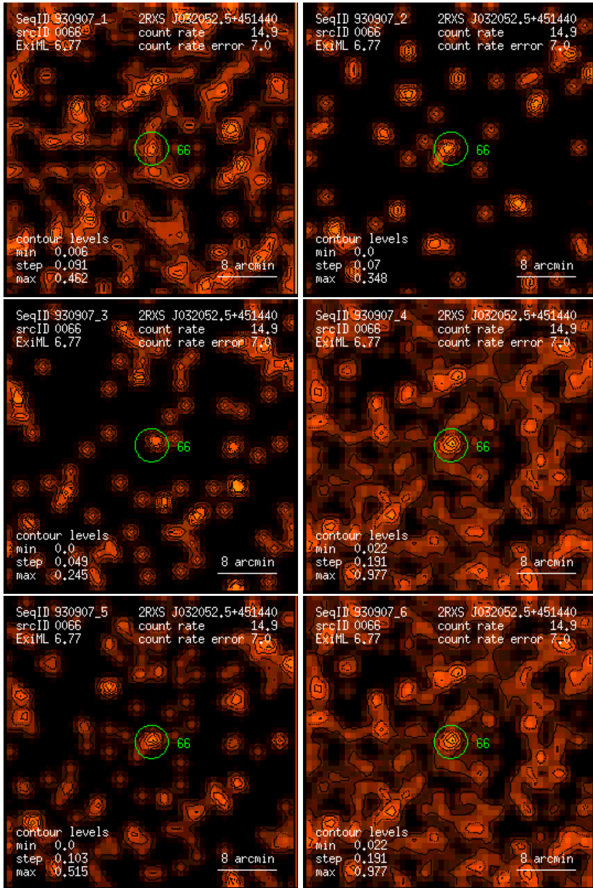
Figure 66: RASS 930907: detection 0066: band rate images, Gaussian filter: (1) PSPC channels 11 – 41, (2) 52 – 90, (3) 91 – 201, (4) 11 – 235, (5) 52 – 201, (6) 11 – 201. Broad band rates in counts/ks. Band rate contour levels in counts/ks/arcmin 2 .
