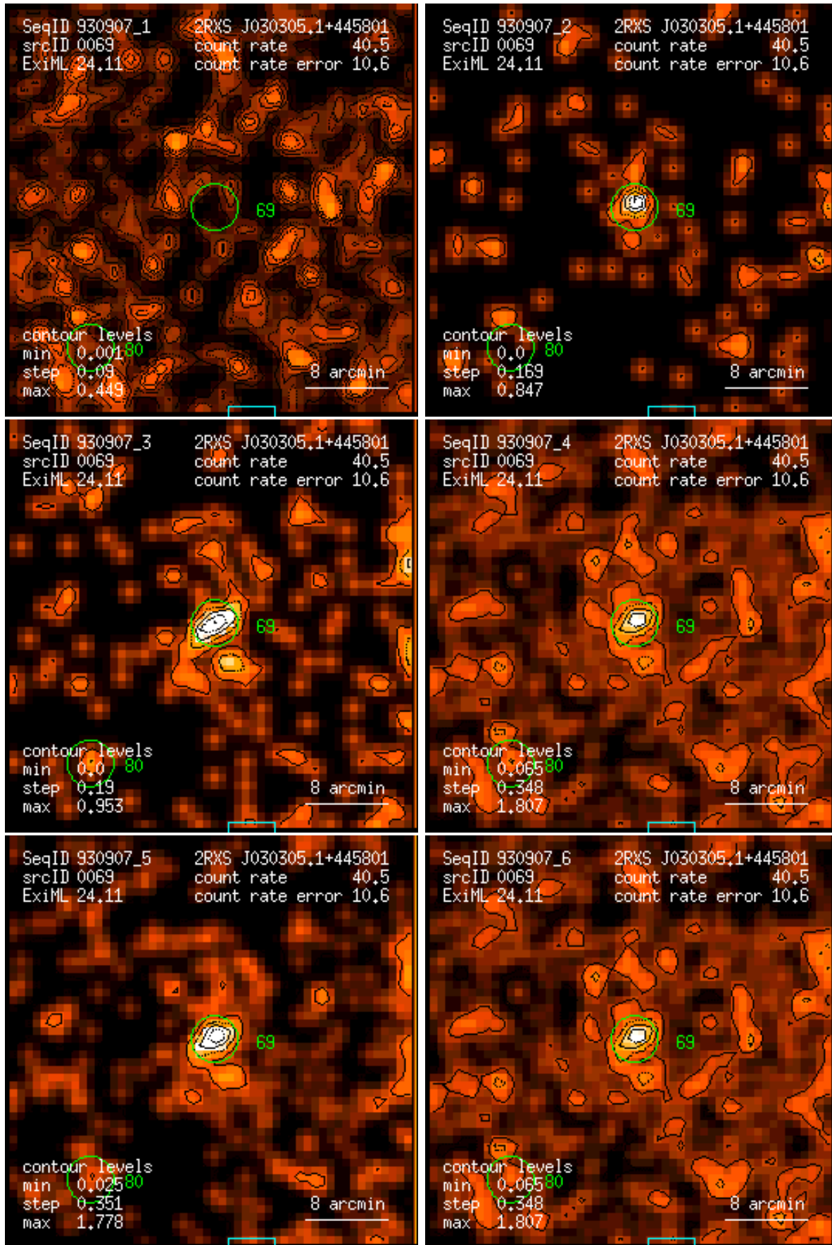
Figure 69: RASS 930907: detection 0069: band rate images, Gaussian filter: (1) PSPC channels 11 – 41, (2) 52 – 90, (3) 91 – 201, (4) 11 – 235, (5) 52 – 201, (6) 11 – 201. Broad band rates in counts/ks. Band rate contour levels in counts/ks/arcmin 2 .
