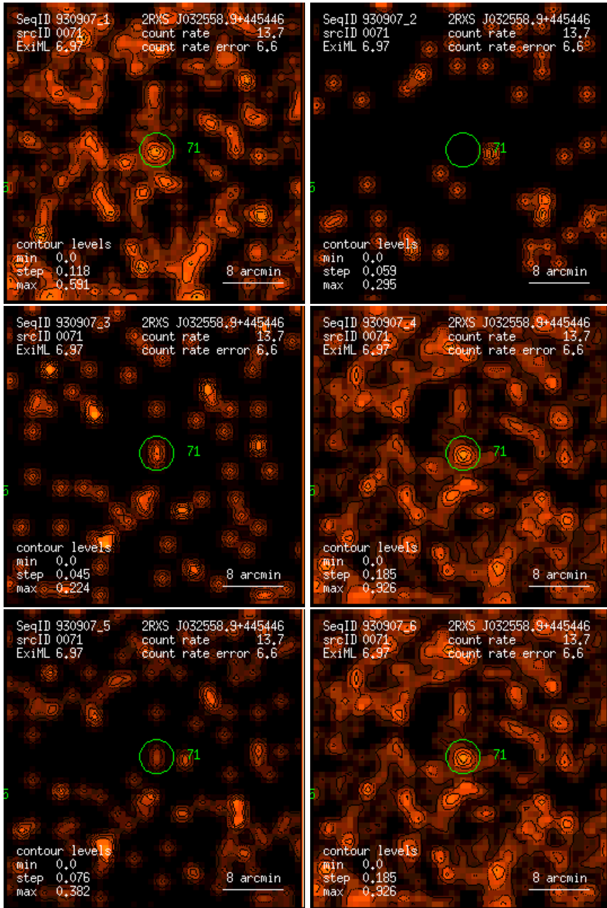
Figure 71: RASS 930907: detection 0071: band rate images, Gaussian filter: (1) PSPC channels 11 – 41, (2) 52 – 90, (3) 91 – 201, (4) 11 – 235, (5) 52 – 201, (6) 11 – 201. Broad band rates in counts/ks. Band rate contour levels in counts/ks/arcmin 2 .
