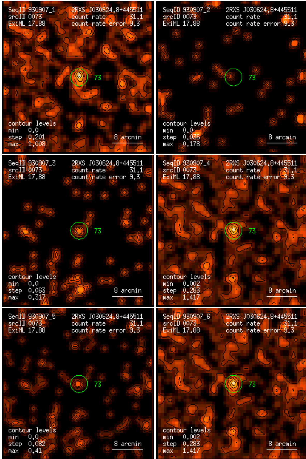
Figure 73: RASS 930907: detection 0073: band rate images, Gaussian filter: (1) PSPC channels 11 – 41, (2) 52 – 90, (3) 91 – 201, (4) 11 – 235, (5) 52 – 201, (6) 11 – 201. Broad band rates in counts/ks. Band rate contour levels in counts/ks/arcmin 2 .
