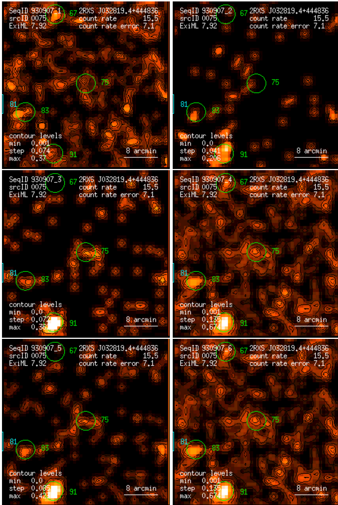
Figure 75: RASS 930907: detection 0075: band rate images, Gaussian filter: (1) PSPC channels 11 – 41, (2) 52 – 90, (3) 91 – 201, (4) 11 – 235, (5) 52 – 201, (6) 11 – 201. Broad band rates in counts/ks. Band rate contour levels in counts/ks/arcmin 2 .
