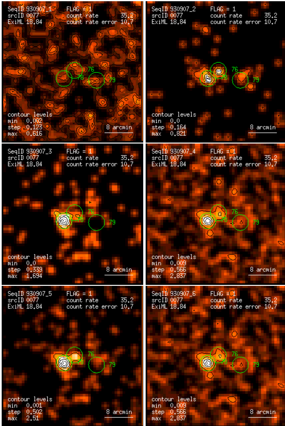
Figure 77: RASS 930907: detection 0077: band rate images, Gaussian filter: (1) PSPC channels 11 – 41, (2) 52 – 90, (3) 91 – 201, (4) 11 – 235, (5) 52 – 201, (6) 11 – 201. Broad band rates in counts/ks. Band rate contour levels in counts/ks/arcmin 2 .
