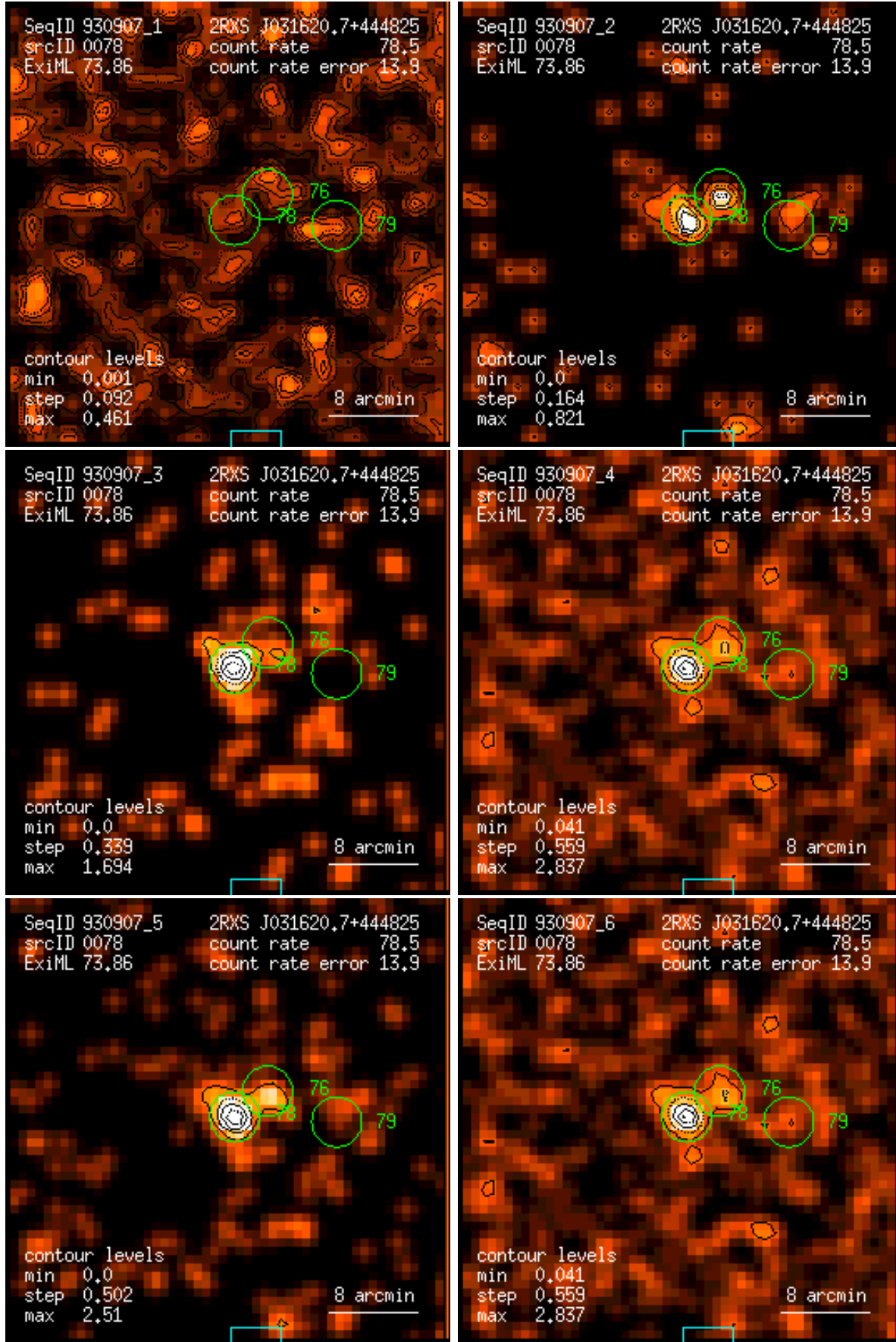
Figure 78: RASS 930907: detection 0078: band rate images, Gaussian filter: (1) PSPC channels 11 – 41, (2) 52 – 90, (3) 91 – 201, (4) 11 – 235, (5) 52 – 201, (6) 11 – 201. Broad band rates in counts/ks. Band rate contour levels in counts/ks/arcmin 2 .
