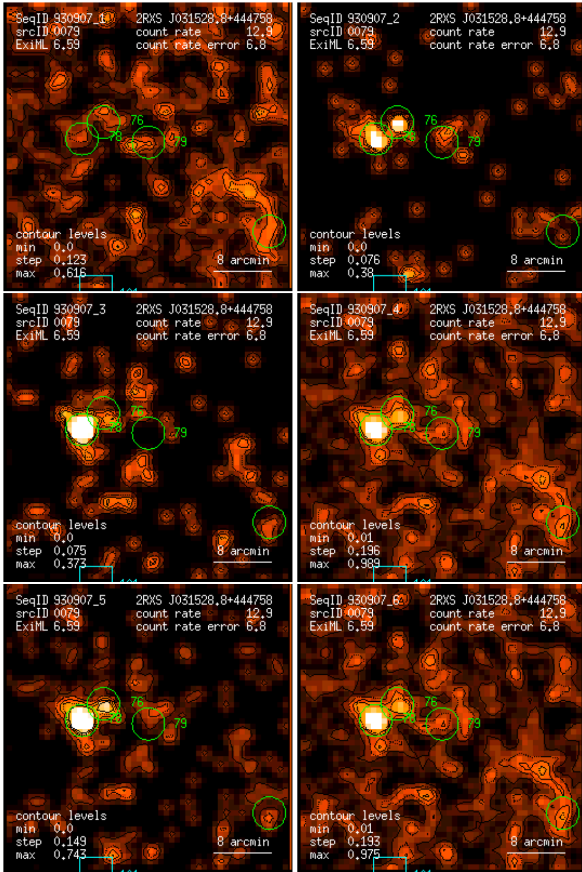
Figure 79: RASS 930907: detection 0079: band rate images, Gaussian filter: (1) PSPC channels 11 – 41, (2) 52 – 90, (3) 91 – 201, (4) 11 – 235, (5) 52 – 201, (6) 11 – 201. Broad band rates in counts/ks. Band rate contour levels in counts/ks/arcmin 2 .
