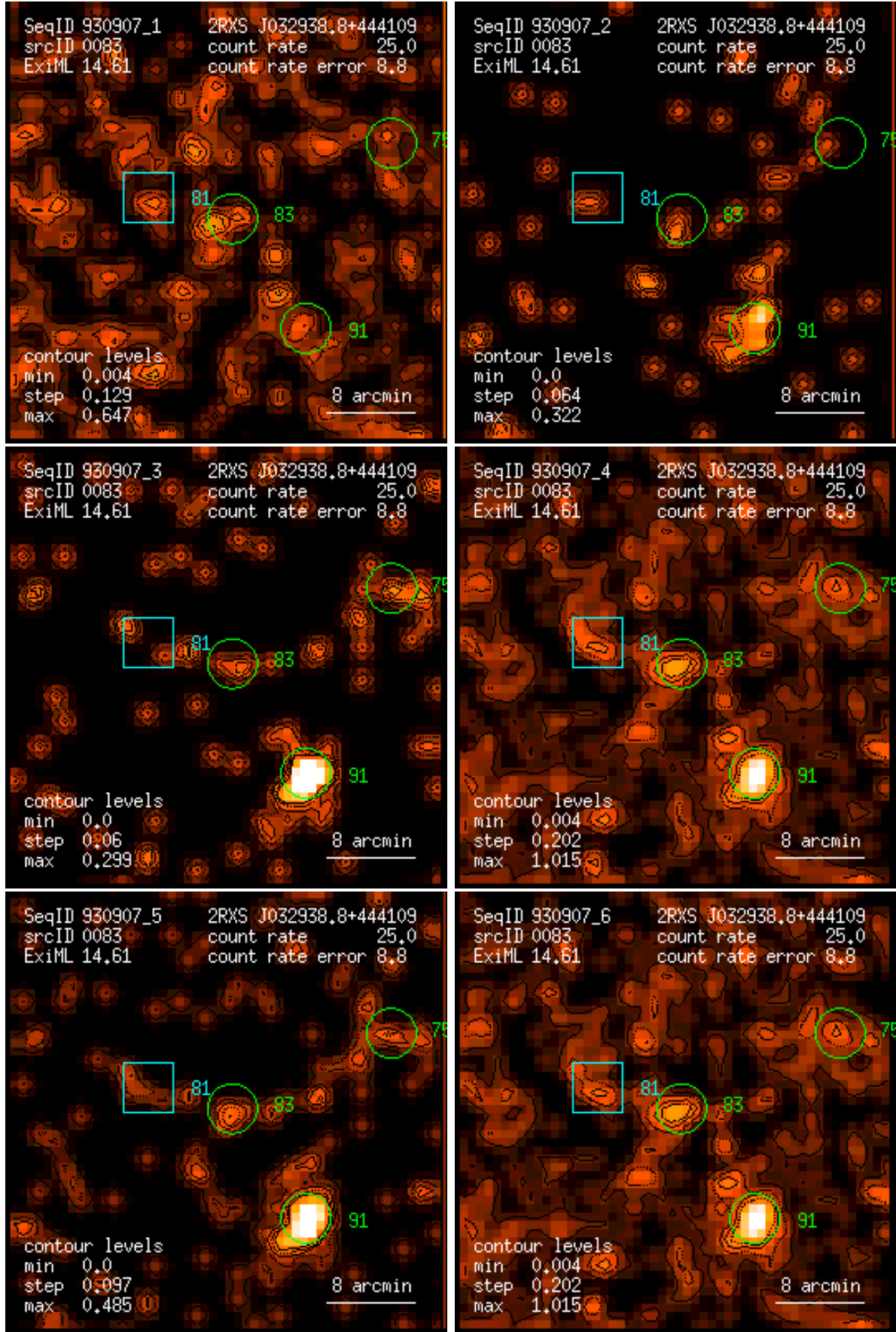
Figure 83: RASS 930907: detection 0083: band rate images, Gaussian filter: (1) PSPC channels 11 – 41, (2) 52 – 90, (3) 91 – 201, (4) 11 – 235, (5) 52 – 201, (6) 11 – 201. Broad band rates in counts/ks. Band rate contour levels in counts/ks/arcmin 2 .
