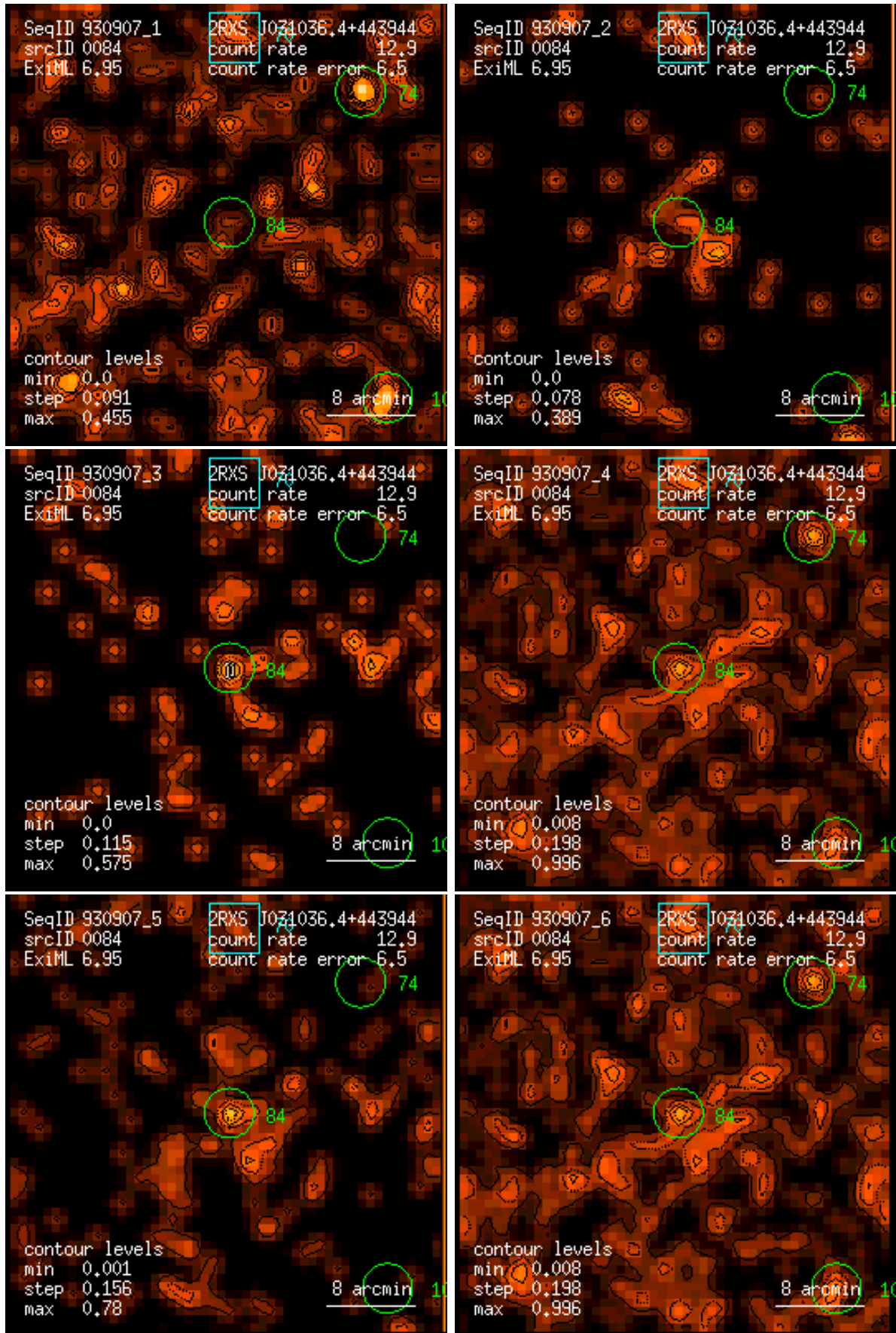
Figure 84: RASS 930907: detection 0084: band rate images, Gaussian filter: (1) PSPC channels 11 – 41, (2) 52 – 90, (3) 91 – 201, (4) 11 – 235, (5) 52 – 201, (6) 11 – 201. Broad band rates in counts/ks. Band rate contour levels in counts/ks/arcmin 2 .
