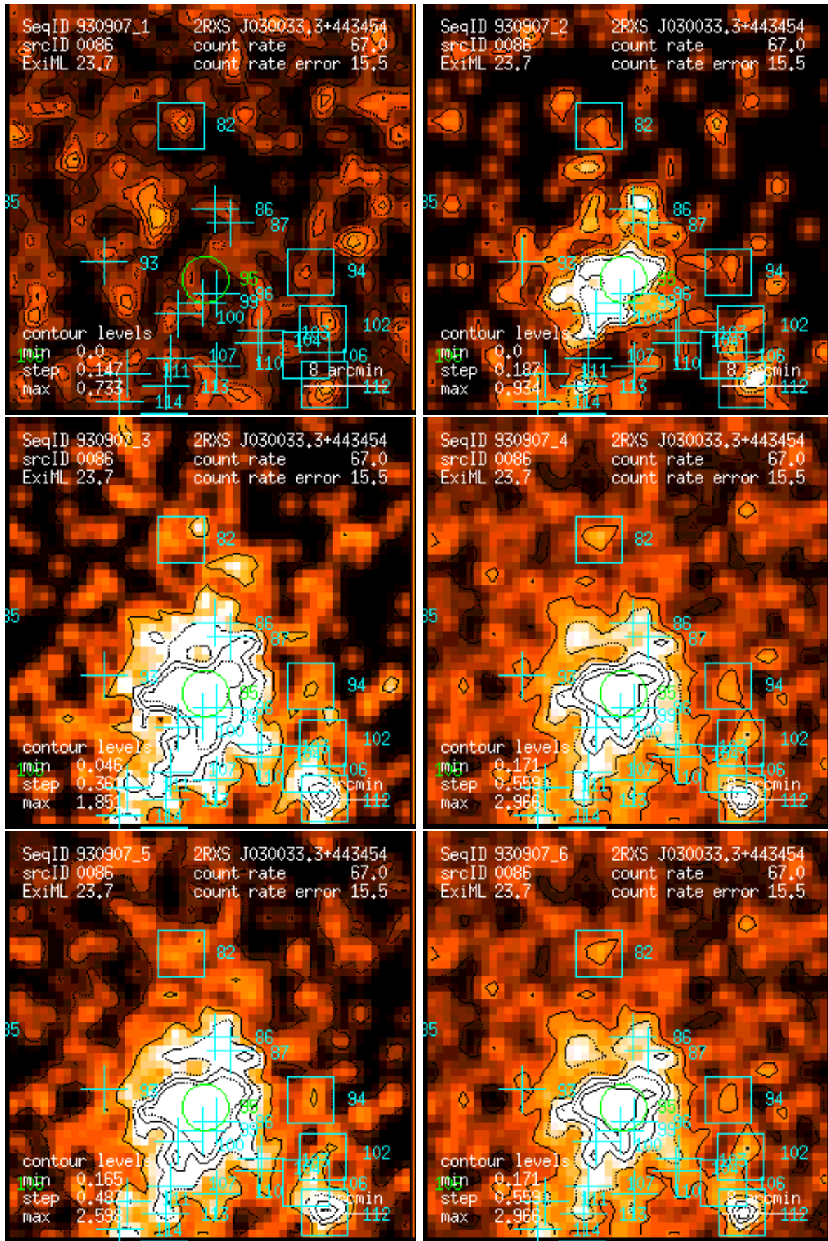
Figure 86: RASS 930907: detection 0086: band rate images, Gaussian filter: (1) PSPC channels 11 – 41, (2) 52 – 90, (3) 91 – 201, (4) 11 – 235, (5) 52 – 201, (6) 11 – 201. Broad band rates in counts/ks. Band rate contour levels in counts/ks/arcmin 2 .
