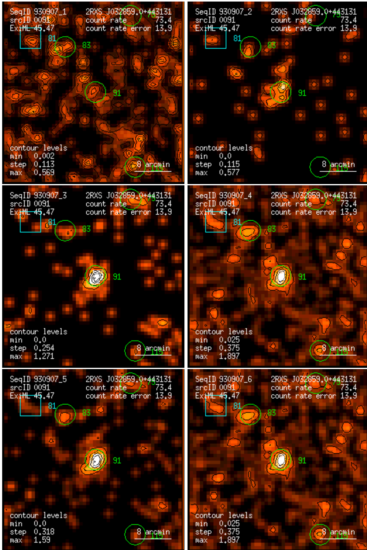
Figure 91: RASS 930907: detection 0091: band rate images, Gaussian filter: (1) PSPC channels 11 – 41, (2) 52 – 90, (3) 91 – 201, (4) 11 – 235, (5) 52 – 201, (6) 11 – 201. Broad band rates in counts/ks. Band rate contour levels in counts/ks/arcmin 2 .
