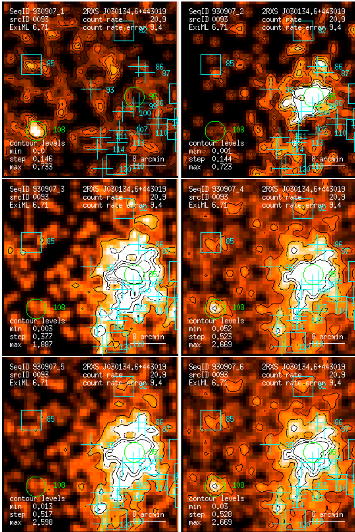
Figure 93: RASS 930907: detection 0093: band rate images, Gaussian filter: (1) PSPC channels 11 – 41, (2) 52 – 90, (3) 91 – 201, (4) 11 – 235, (5) 52 – 201, (6) 11 – 201. Broad band rates in counts/ks. Band rate contour levels in counts/ks/arcmin 2 .
