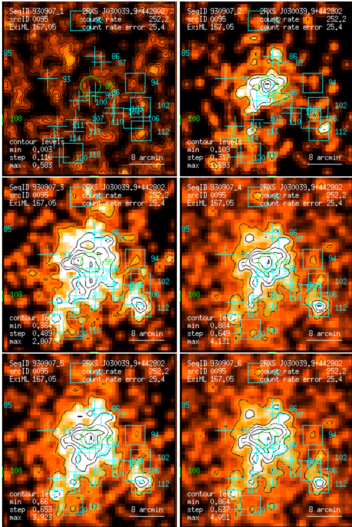
Figure 95: RASS 930907: detection 0095: band rate images, Gaussian filter: (1) PSPC channels 11 – 41, (2) 52 – 90, (3) 91 – 201, (4) 11 – 235, (5) 52 – 201, (6) 11 – 201. Broad band rates in counts/ks. Band rate contour levels in counts/ks/arcmin 2 .
