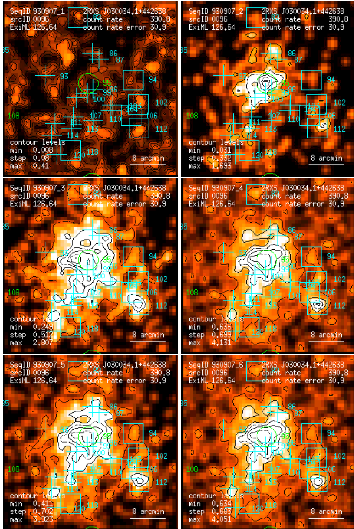
Figure 96: RASS 930907: detection 0096: band rate images, Gaussian filter: (1) PSPC channels 11 – 41, (2) 52 – 90, (3) 91 – 201, (4) 11 – 235, (5) 52 – 201, (6) 11 – 201. Broad band rates in counts/ks. Band rate contour levels in counts/ks/arcmin 2 .
