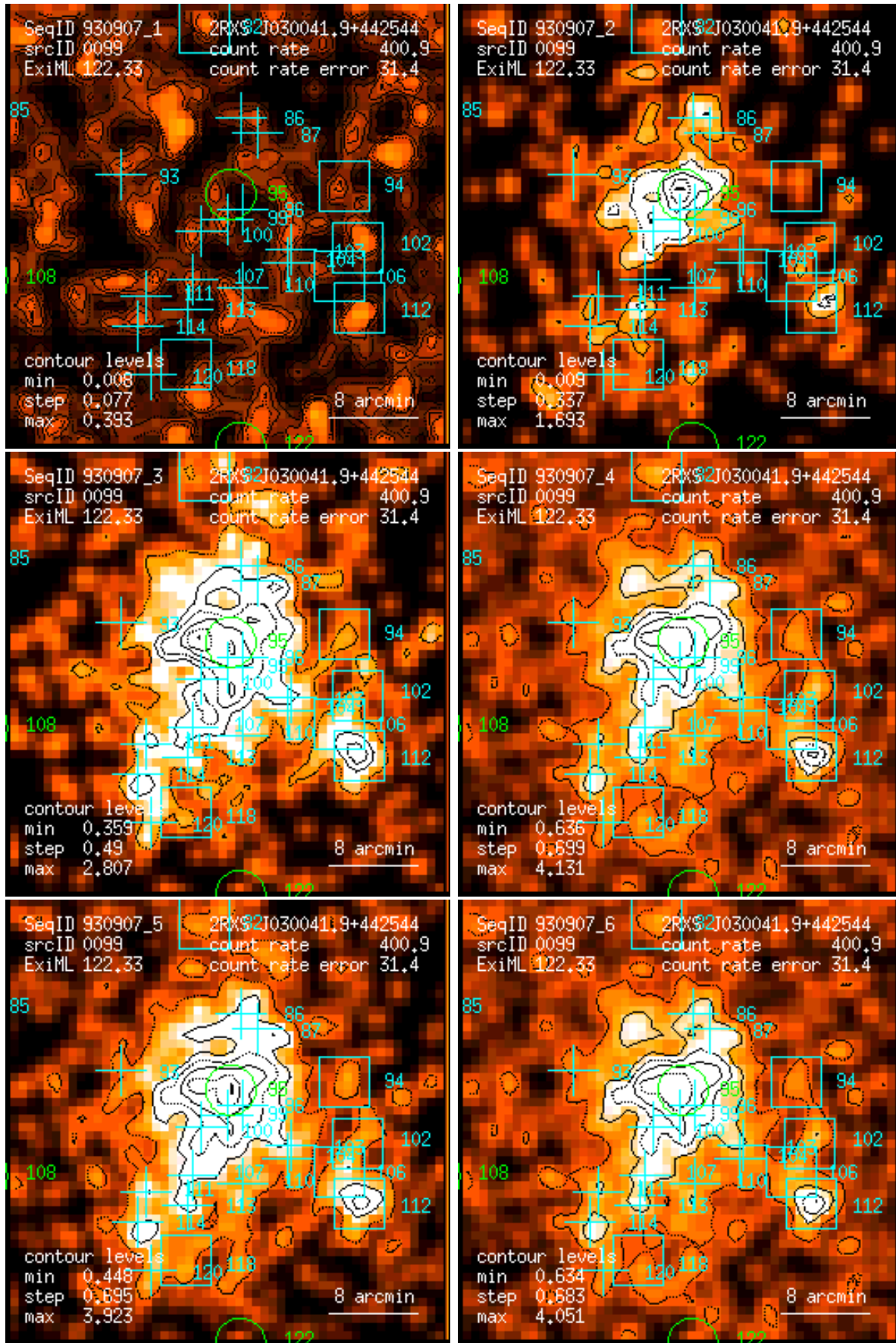
Figure 99: RASS 930907: detection 0099: band rate images, Gaussian filter: (1) PSPC channels 11 – 41, (2) 52 – 90, (3) 91 – 201, (4) 11 – 235, (5) 52 – 201, (6) 11 – 201. Broad band rates in counts/ks. Band rate contour levels in counts/ks/arcmin 2 .
