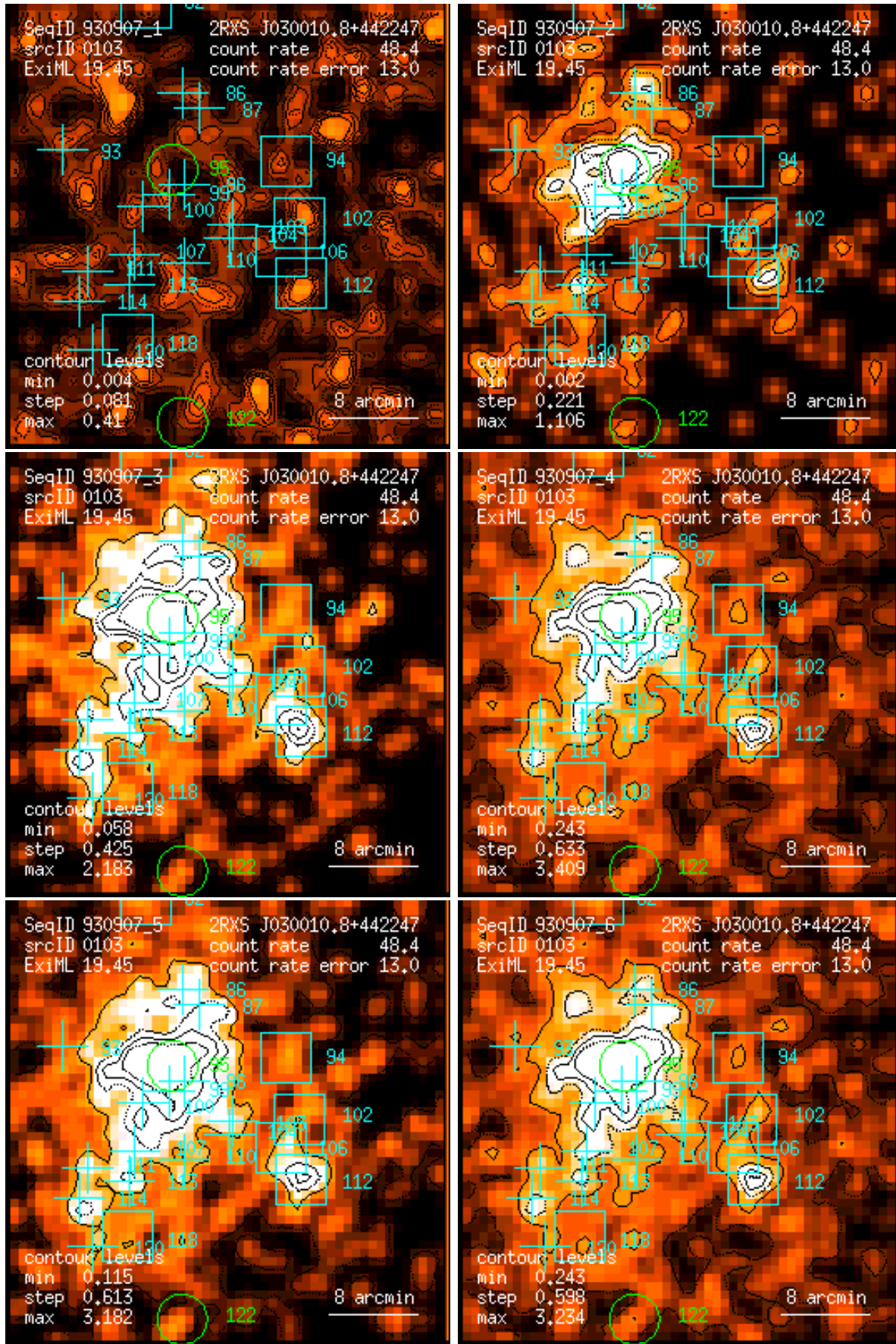
Figure 103: RASS 930907: detection 0103: band rate images, Gaussian filter: (1) PSPC channels 11 – 41, (2) 52 – 90, (3) 91 – 201, (4) 11 – 235, (5) 52 – 201, (6) 11 – 201. Broad band rates in counts/ks. Band rate contour levels in counts/ks/arcmin 2 .
