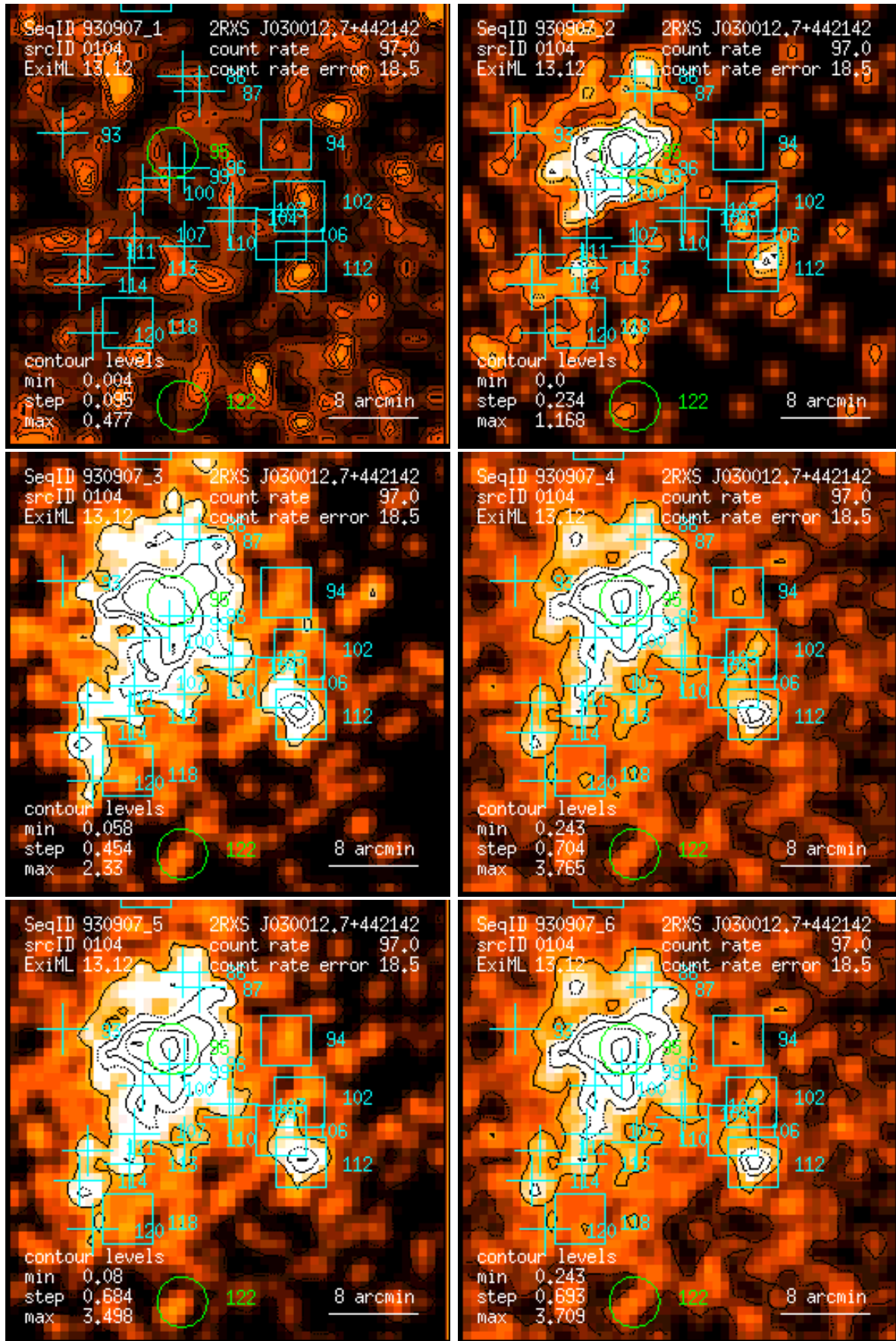
Figure 104: RASS 930907: detection 0104: band rate images, Gaussian filter: (1) PSPC channels 11 – 41, (2) 52 – 90, (3) 91 – 201, (4) 11 – 235, (5) 52 – 201, (6) 11 – 201. Broad band rates in counts/ks. Band rate contour levels in counts/ks/arcmin 2 .
