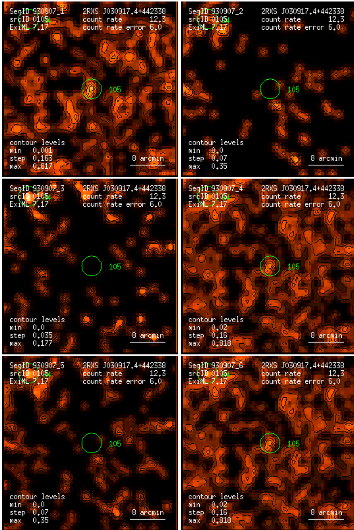
Figure 105: RASS 930907: detection 0105: band rate images, Gaussian filter: (1) PSPC channels 11 – 41, (2) 52 – 90, (3) 91 – 201, (4) 11 – 235, (5) 52 – 201, (6) 11 – 201. Broad band rates in counts/ks. Band rate contour levels in counts/ks/arcmin 2 .
