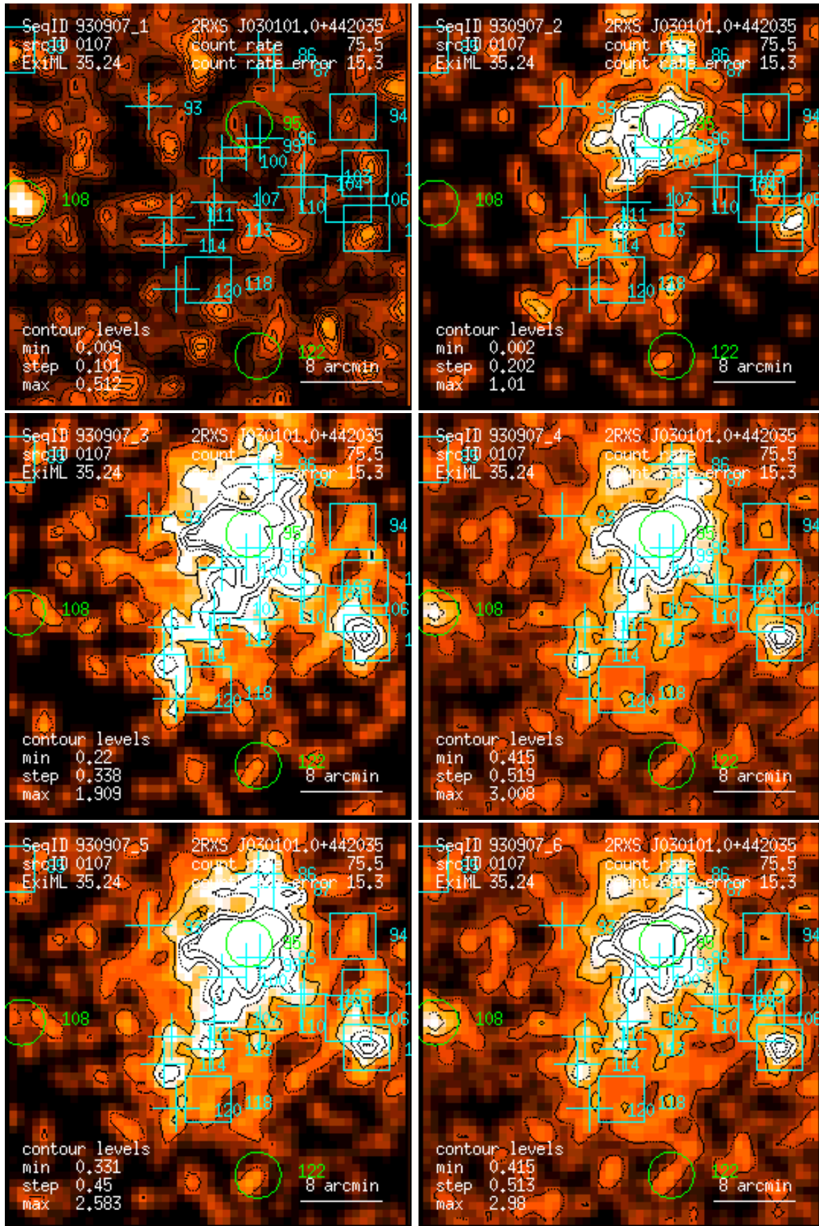
Figure 107: RASS 930907: detection 0107: band rate images, Gaussian filter: (1) PSPC channels 11 – 41, (2) 52 – 90, (3) 91 – 201, (4) 11 – 235, (5) 52 – 201, (6) 11 – 201. Broad band rates in counts/ks. Band rate contour levels in counts/ks/arcmin 2 .
